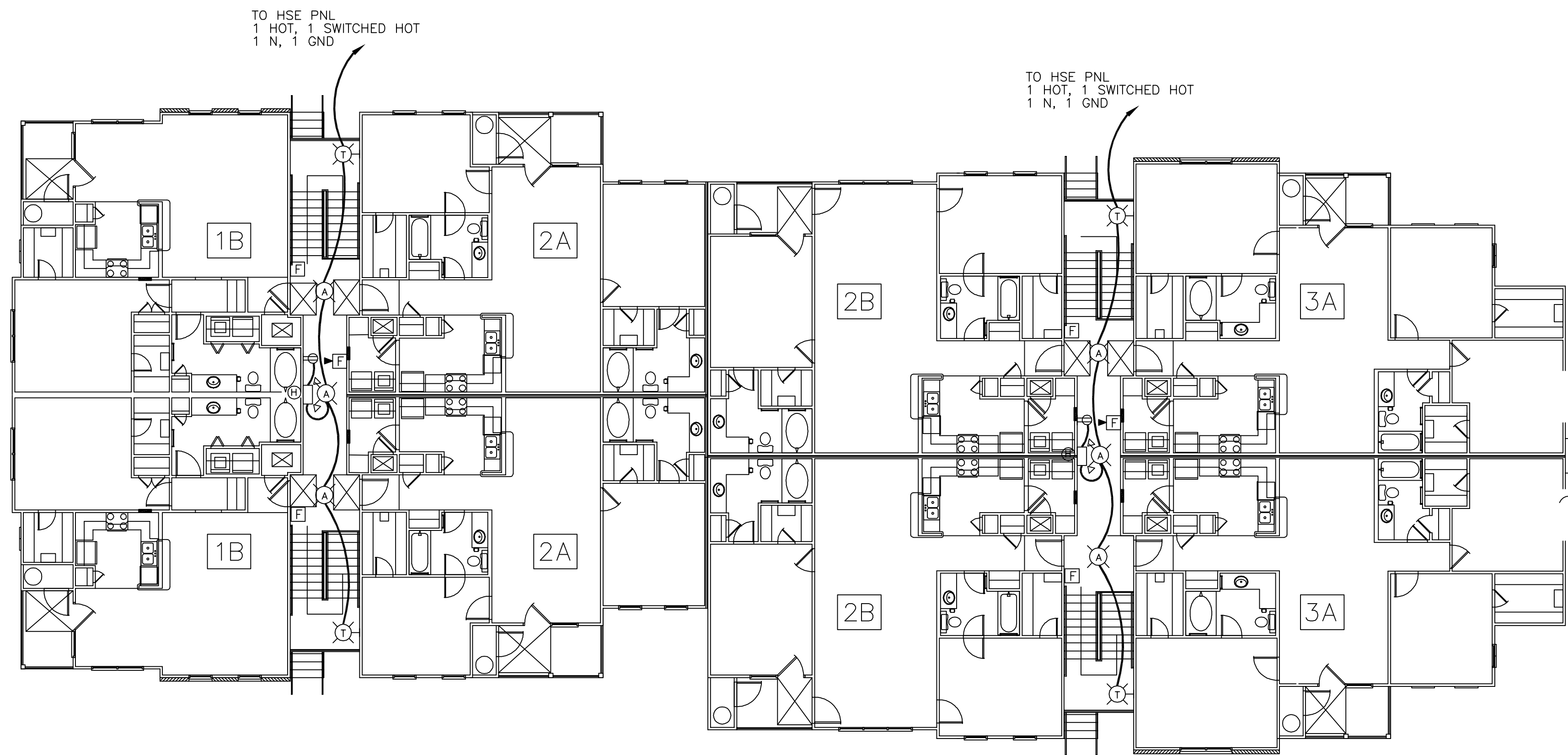
BLDG #2 SECOND & THIRD FLOOR LIGHTING & POWER SCALE: 1/8" = 1'-0"
