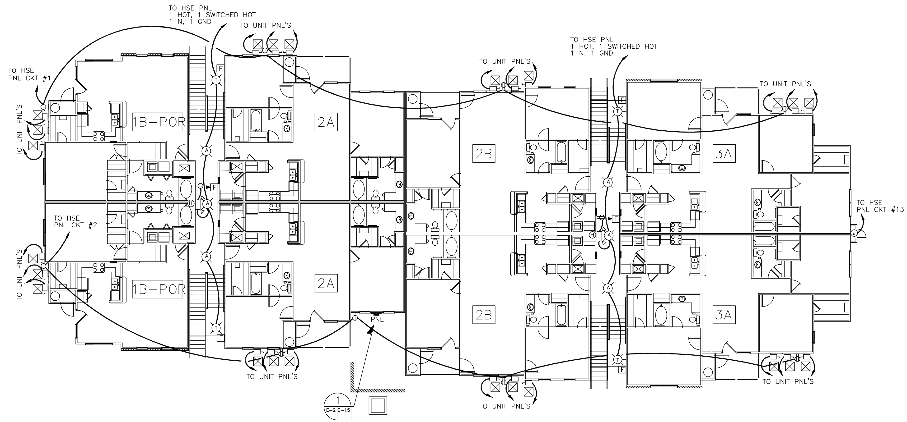
BLDG #2 FIRST FLOOR LIGHTING & POWER SCALE: 1/8" = 1'-0"
