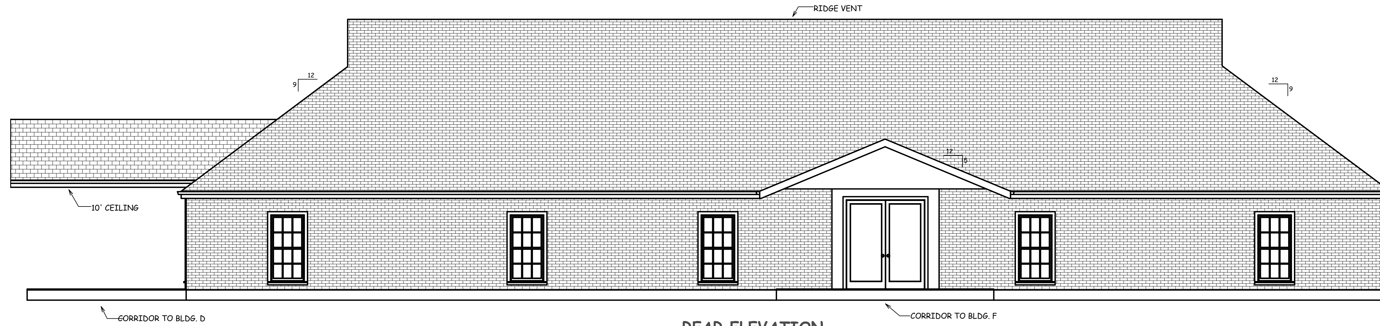
REAR ELEVATION
