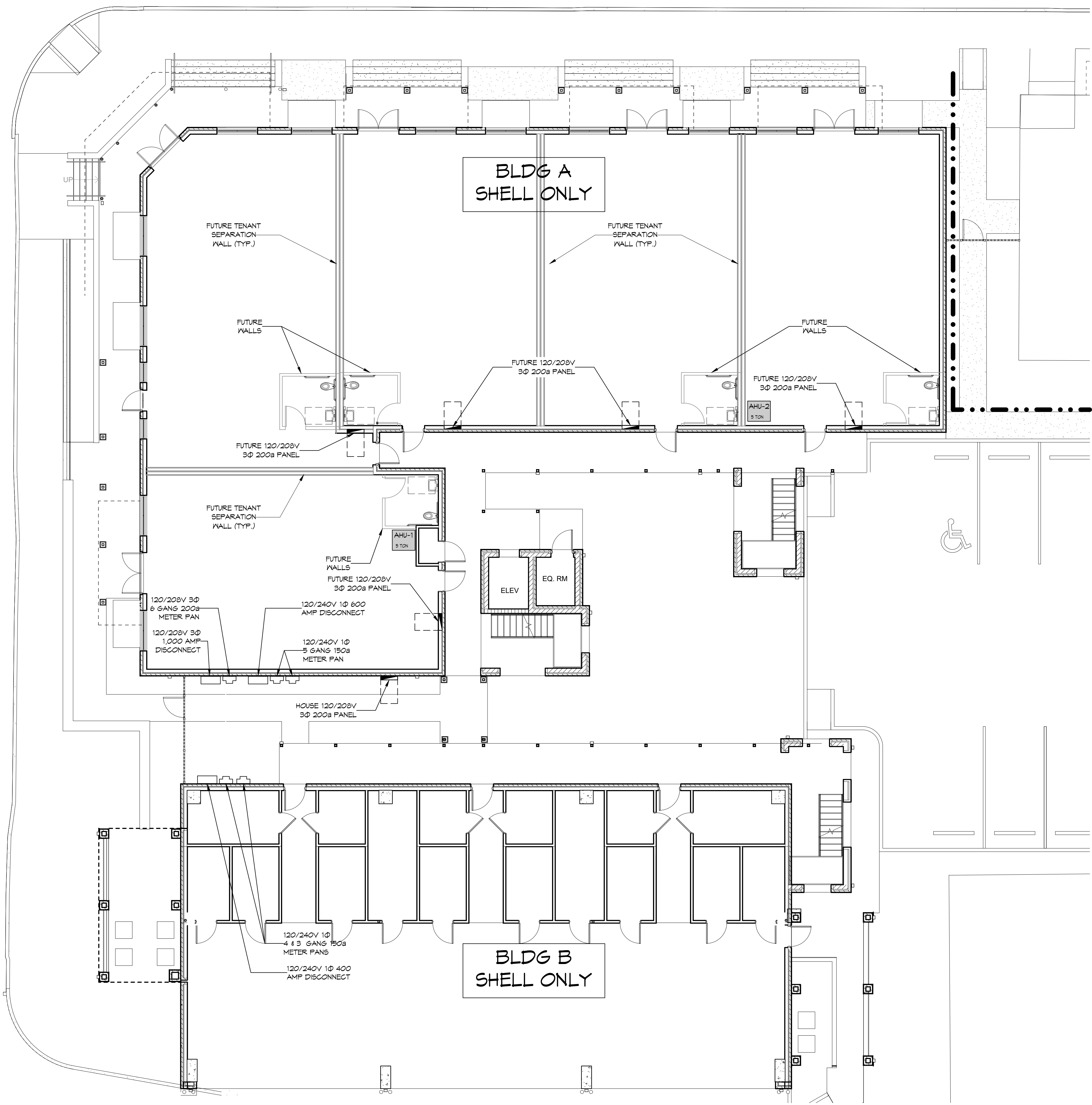
1 FIRST FLOOR MECHANICAL PLAN SCALE: 1/8" = 1'-0"
