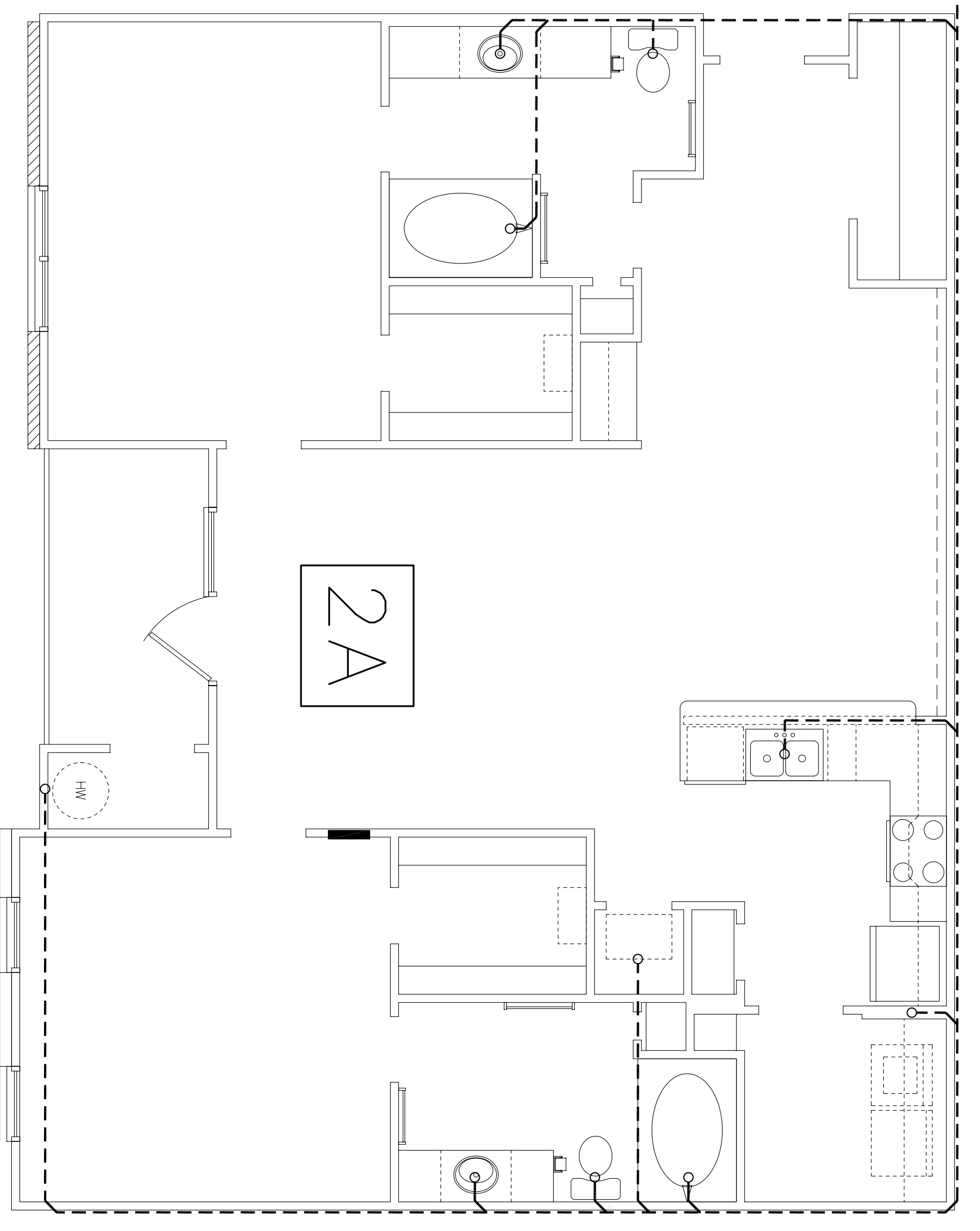
UNIT 2A SEWER PLUMBING RISER SCALE: 1/4" = 1'-0"
