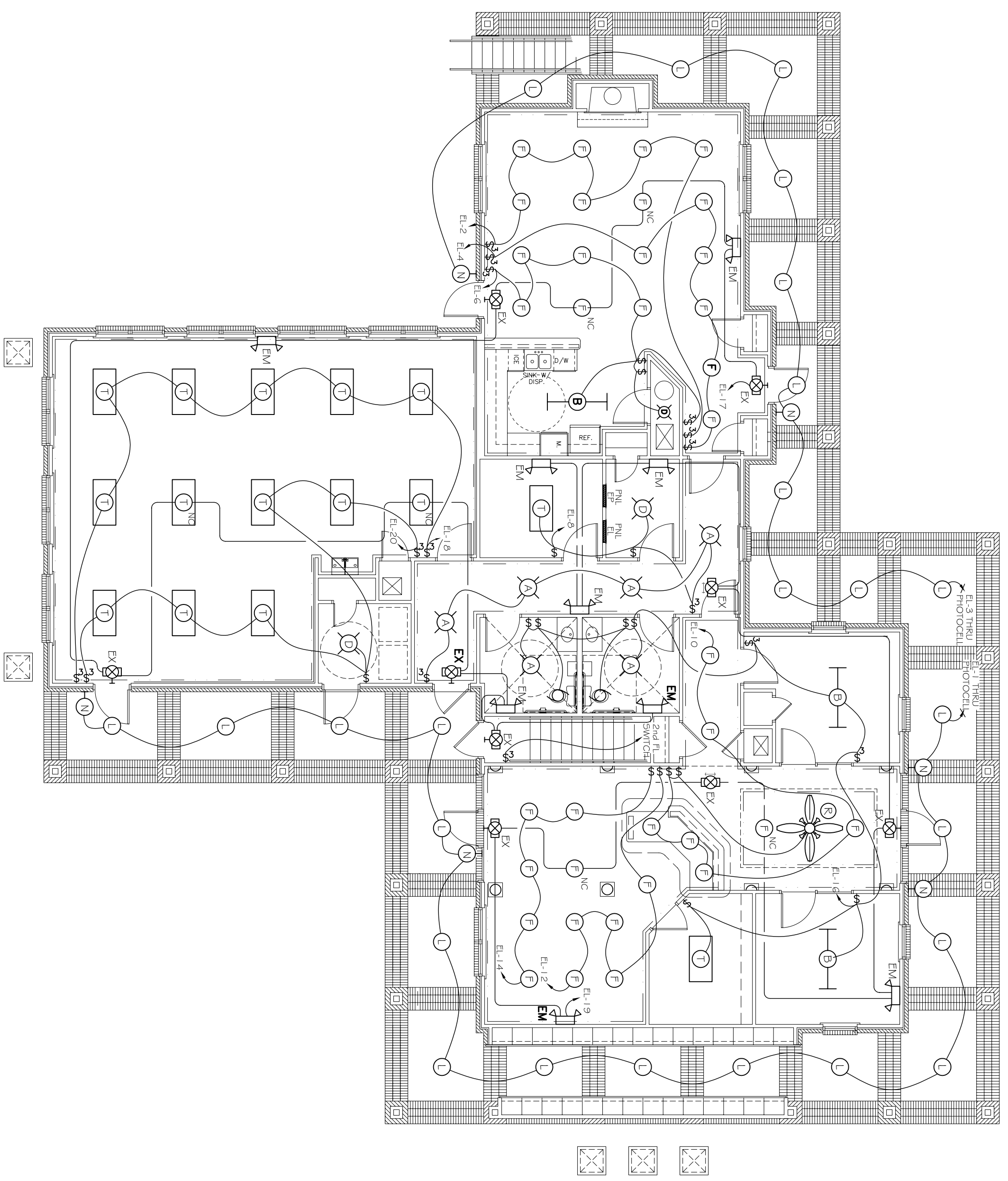
LEASING BLDG. 1ST FLOOR LIGHTING PLAN SCALE: 1/8" = 1'-0"
