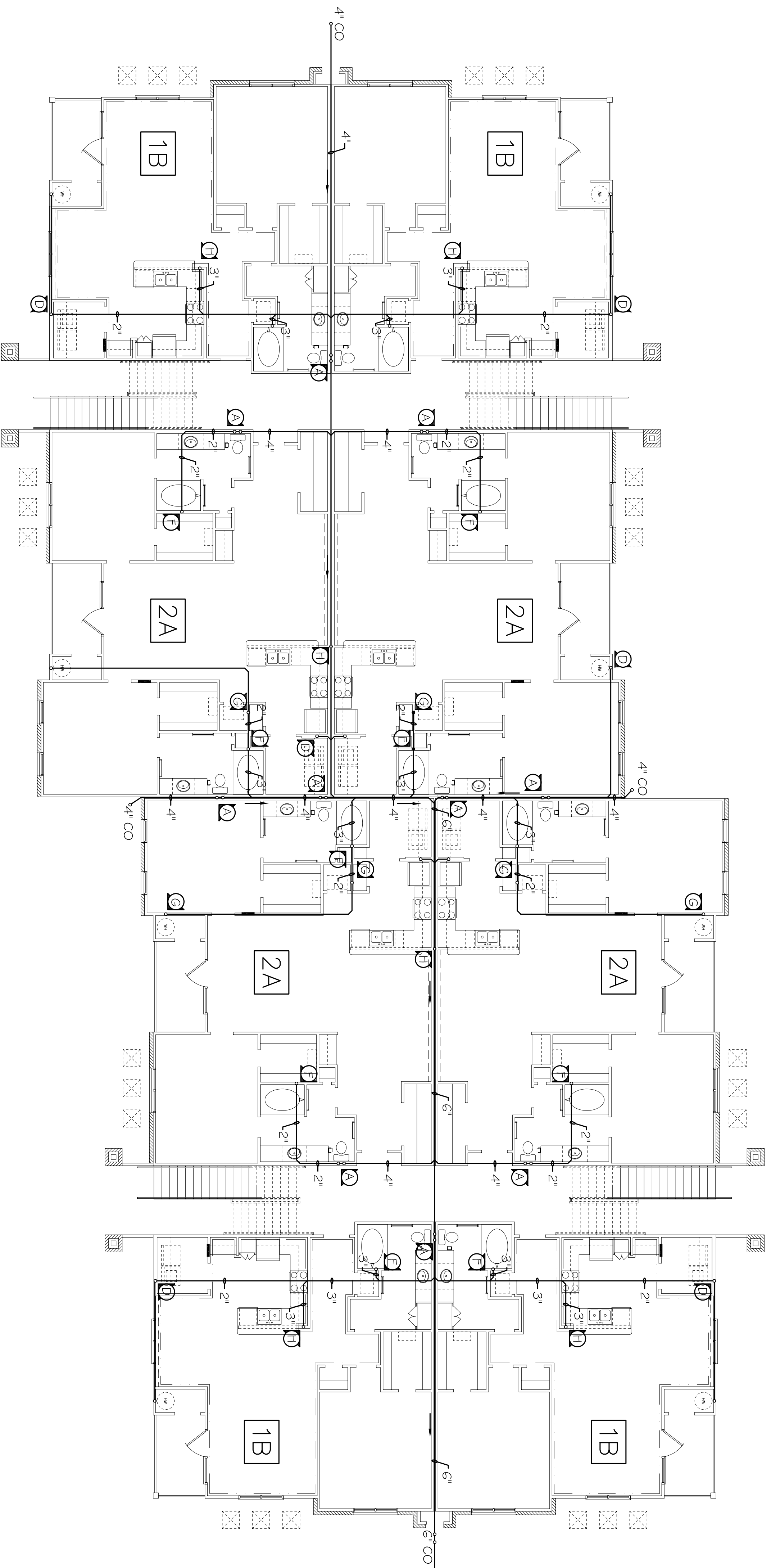
BLDG. 3 1ST FLOOR PLUMBING PLAN SCALE: 1/8"=1'-0"
