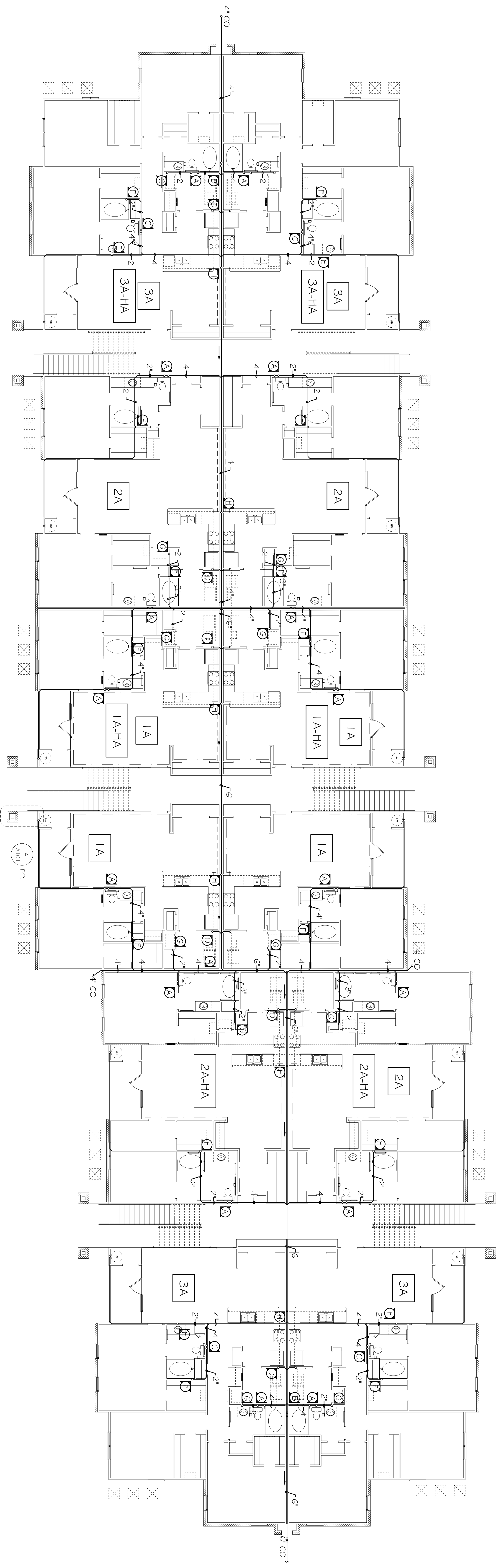
BLDG. 1, 2, 5 & 6 1ST FLOOR PLUMBING PLAN SCALE: 1/8"=1'-0"
