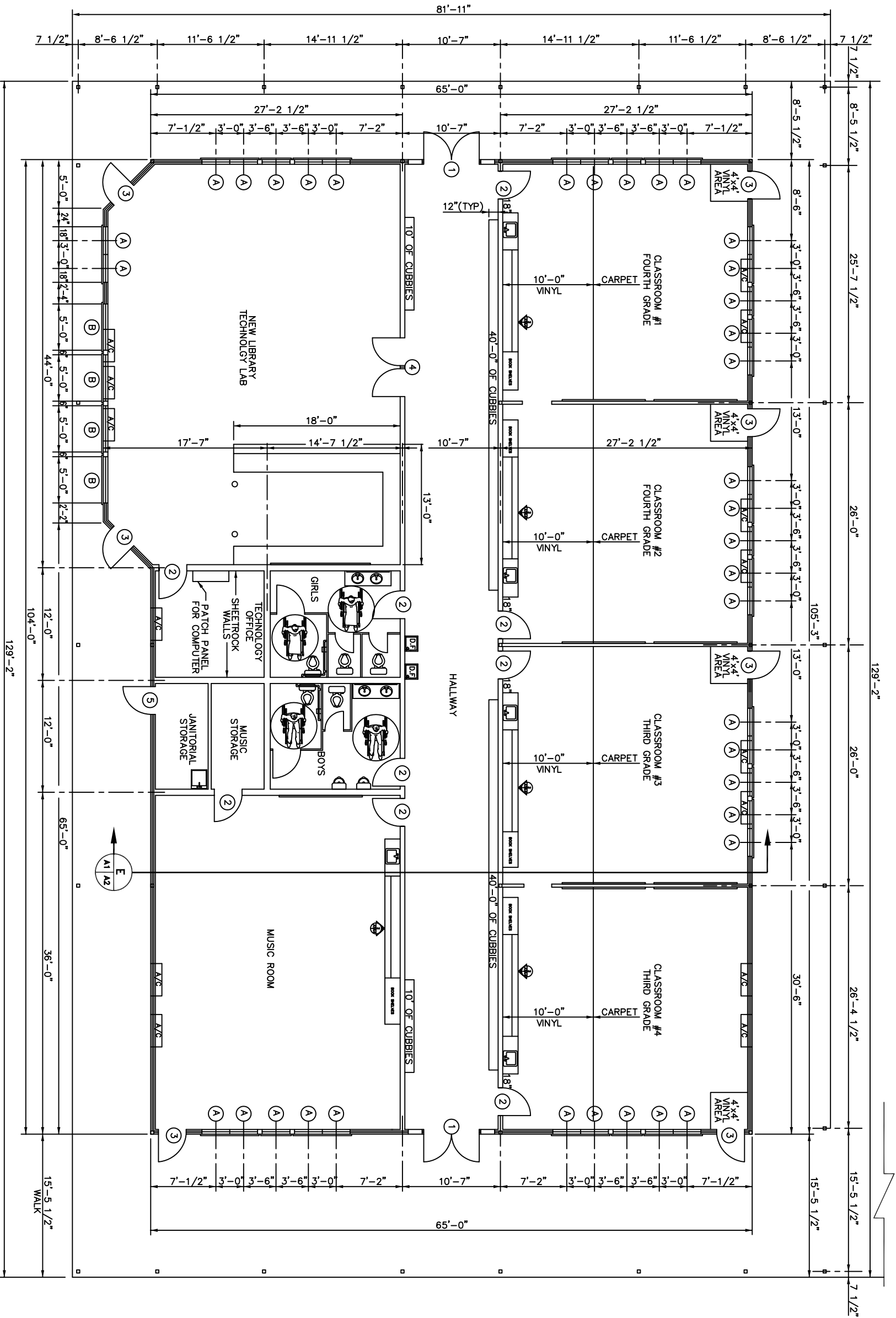
FLOOR PLAN SCALE: 3/16"=1'-0"
