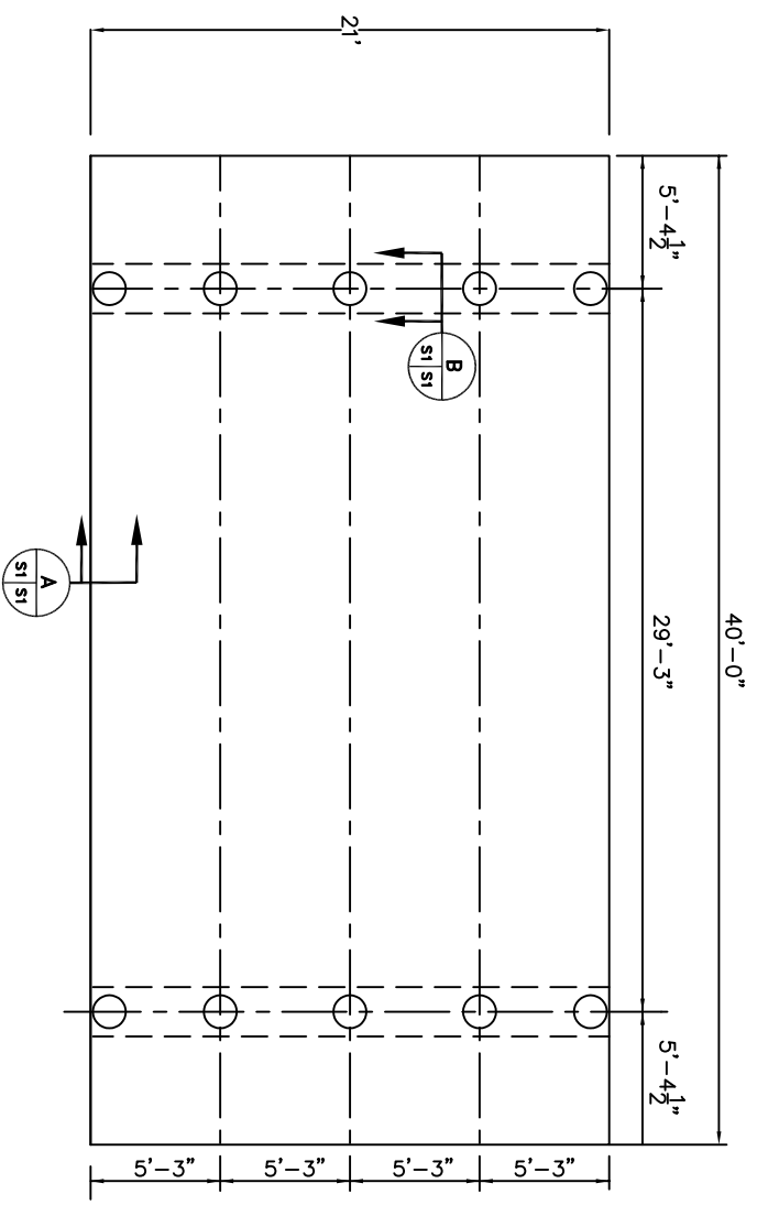
FOUNDATION PLAN SCALE: 1/4"=1'-0"
