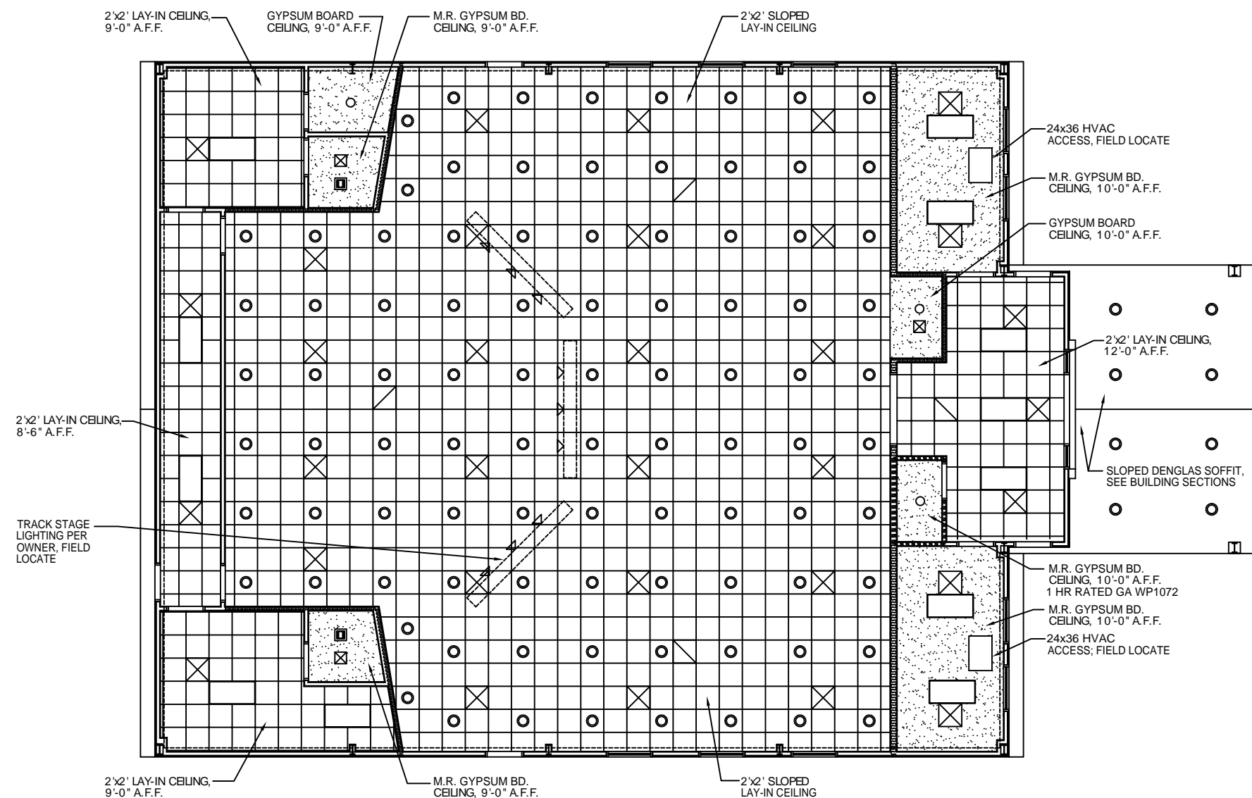
REFLECTED CEILING PLAN SCALE: 3/16"=1'
