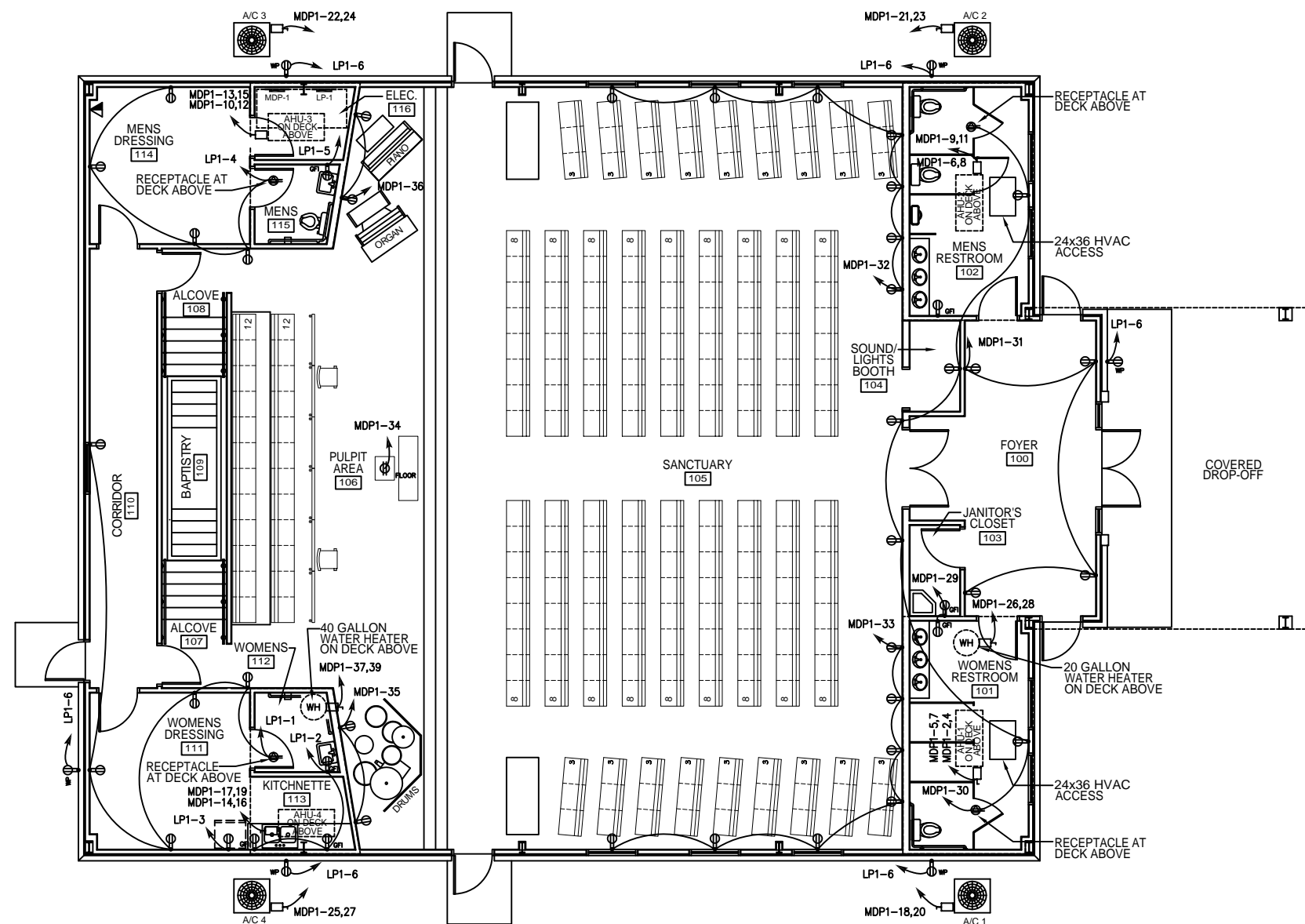
ELECTRICAL POWER PLAN SCALE: 3/16"=1'
