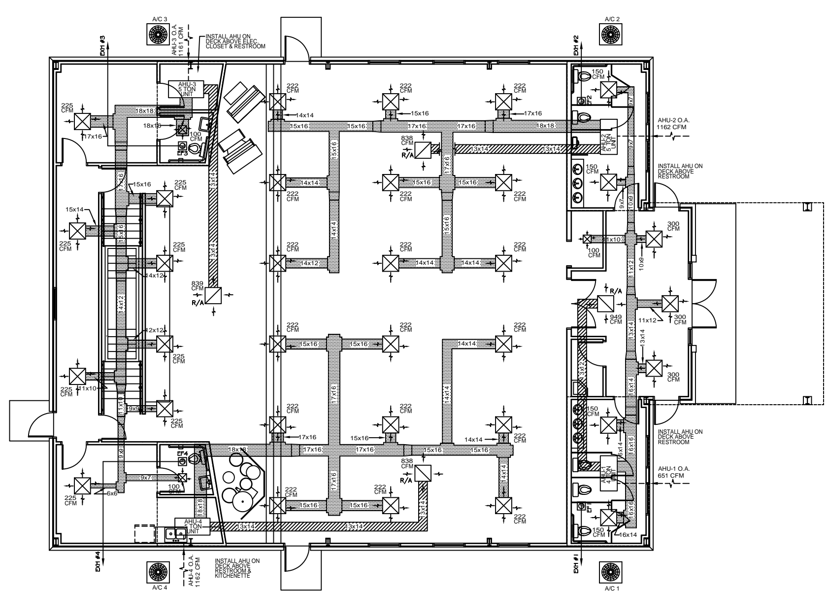
MECHANICAL PLAN SCALE: 3/16"=1'
