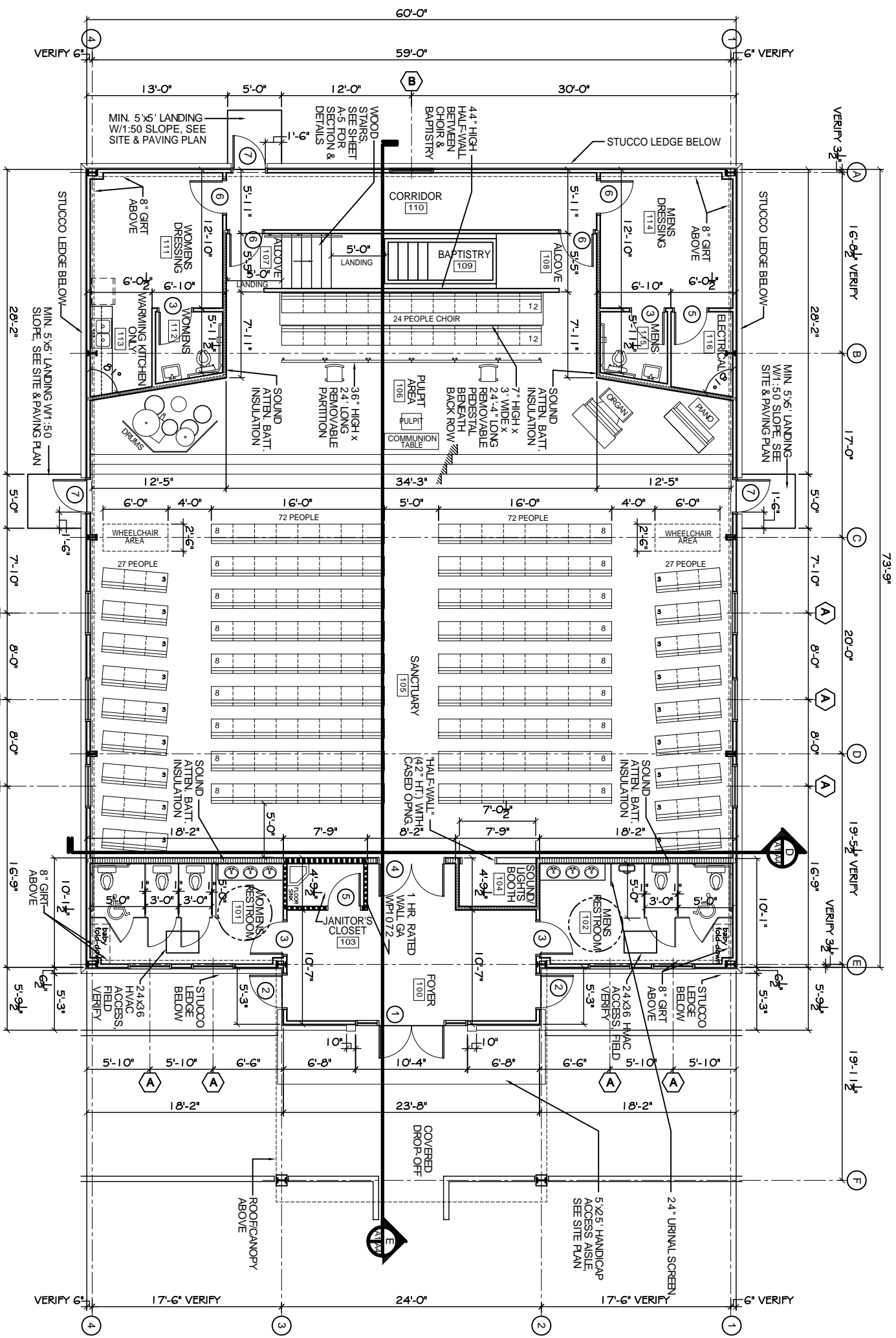
FLOOR PLAN SCALE: 3/16" = 1'
