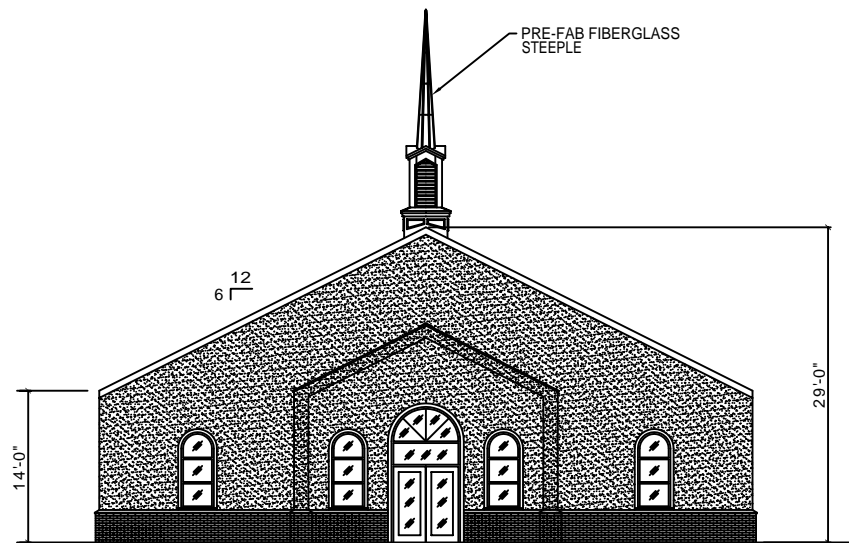
FRONT ELEVATION SCALE: 1/8"=1'
