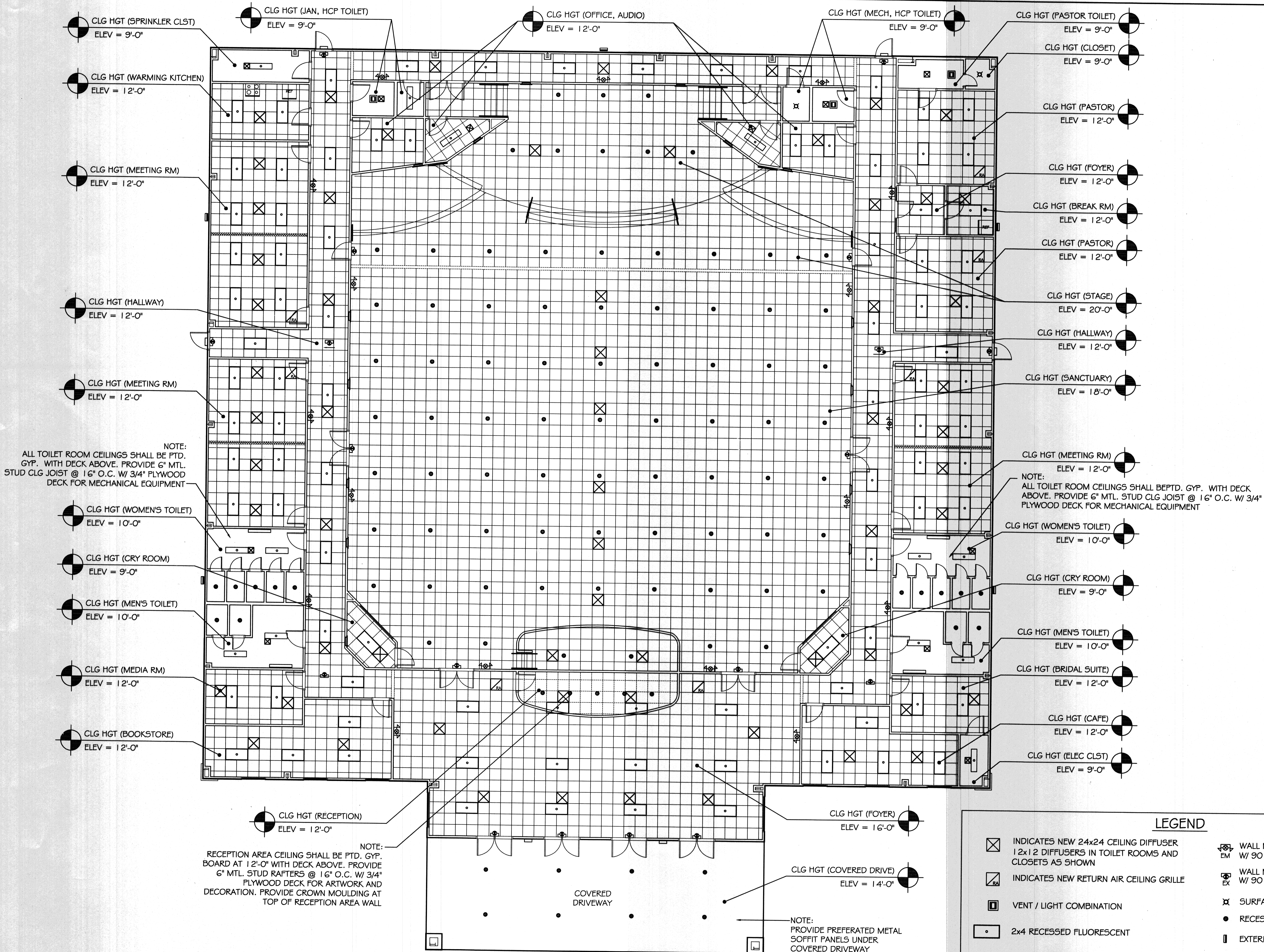
REFLECTED CEILING PLAN
