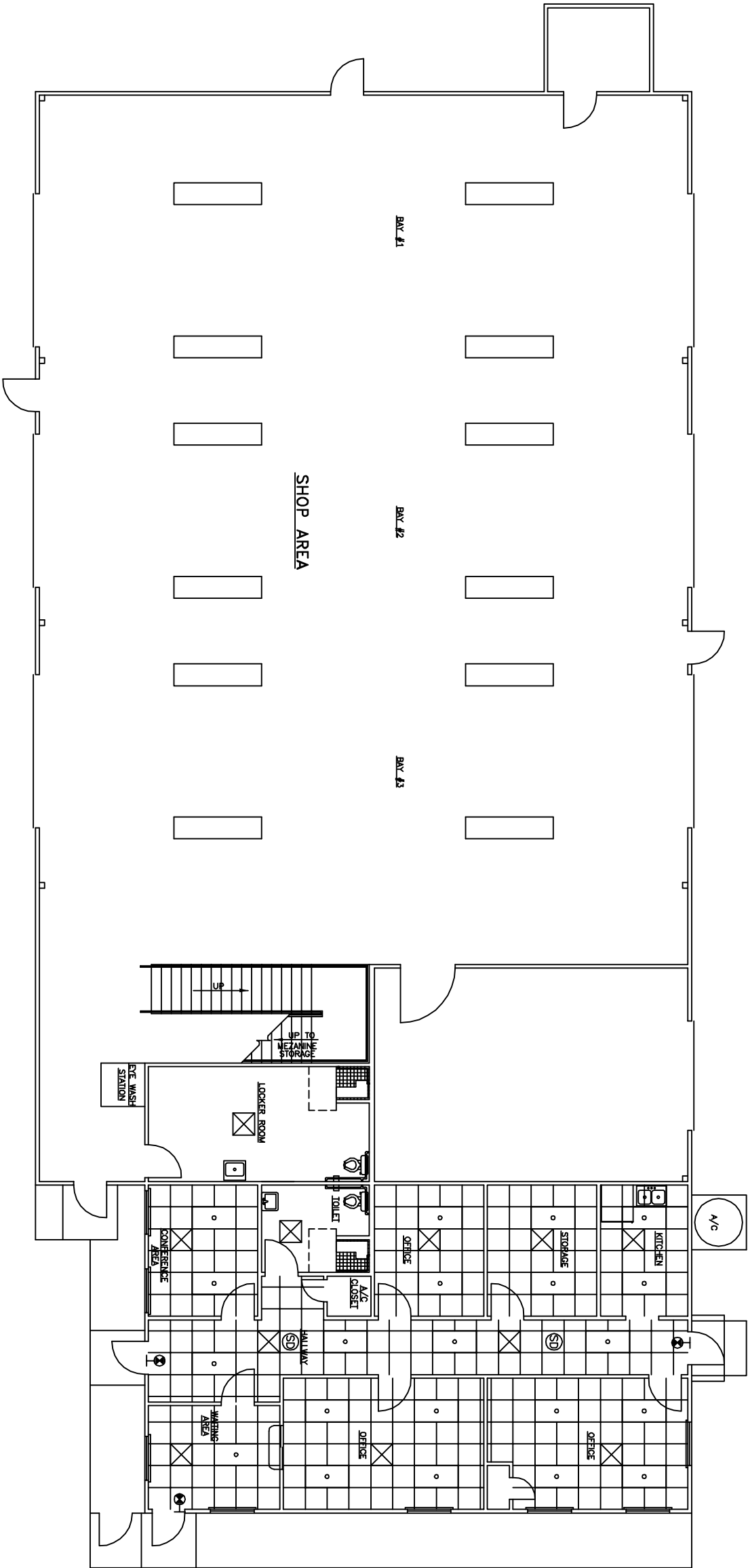
REFLECTED CEILING PLAN SCALE: 3/16"=1'-0"
