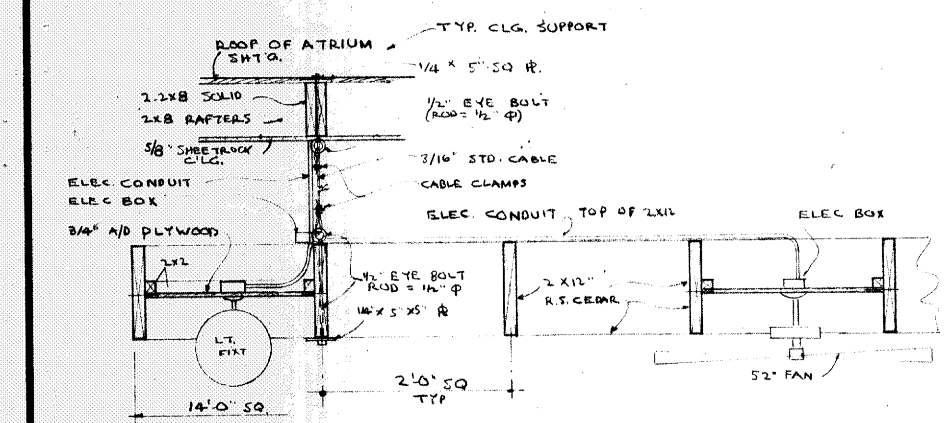
SEC. THRU SUSPENDED ITEMS 1 & 2 SCALE 1" = 1'-0"
