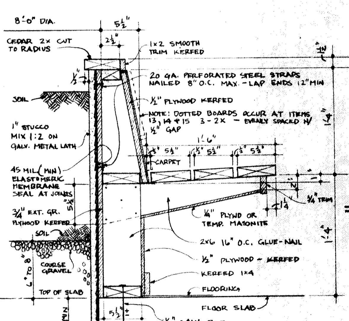
SEC.-ITEM #9 (ALSO ITEMS #13, 14 + 15) SCALE 1 1/2" = 1'-0"
