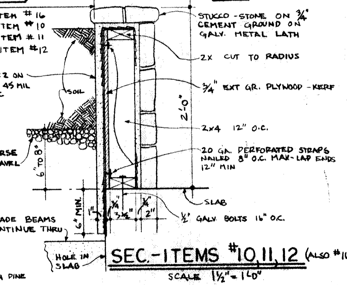
SEC.-ITEMS #10, 11, 12 (ALSO #16) SCALE 1/2" = 1'-0"
