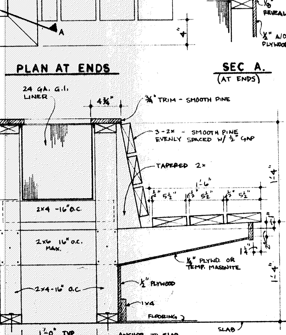
SEC.-ITEMS #21 & 22 SCALE 1 1/2" = 1'-0"
