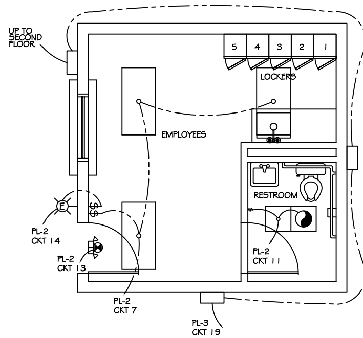
FIRST FLOOR LIGHTING PLAN SCALE: 3/8"=1'-0"
