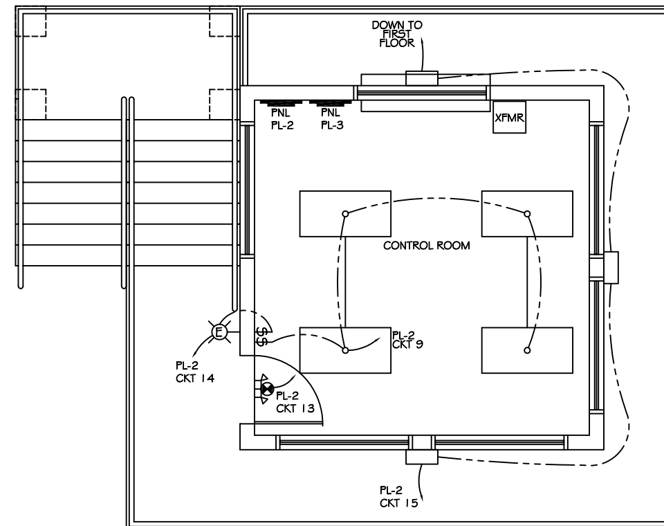
SECOND FLOOR LIGHTING PLAN SCALE: 3/8"=1'-0"
