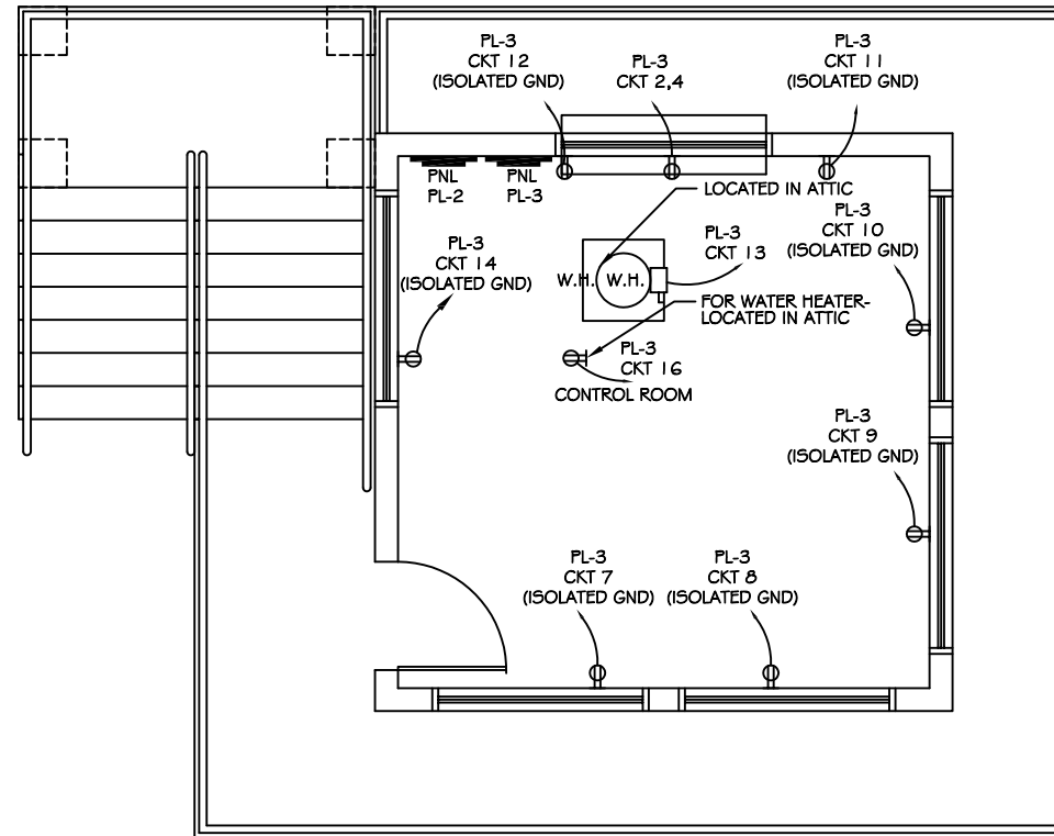
SECOND FLOOR POWER PLAN SCALE: 3/8"=1'-0"
