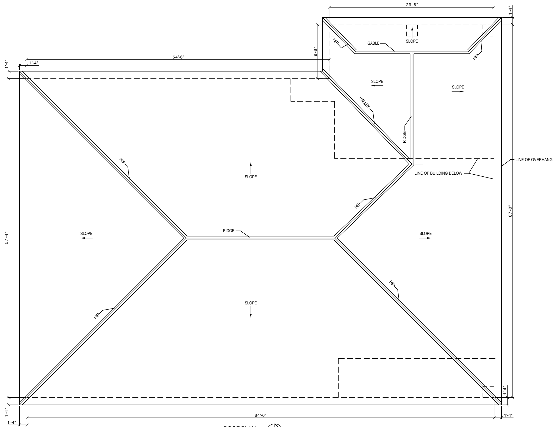
ROOF PLAN SCALE: 1/4"=1'
