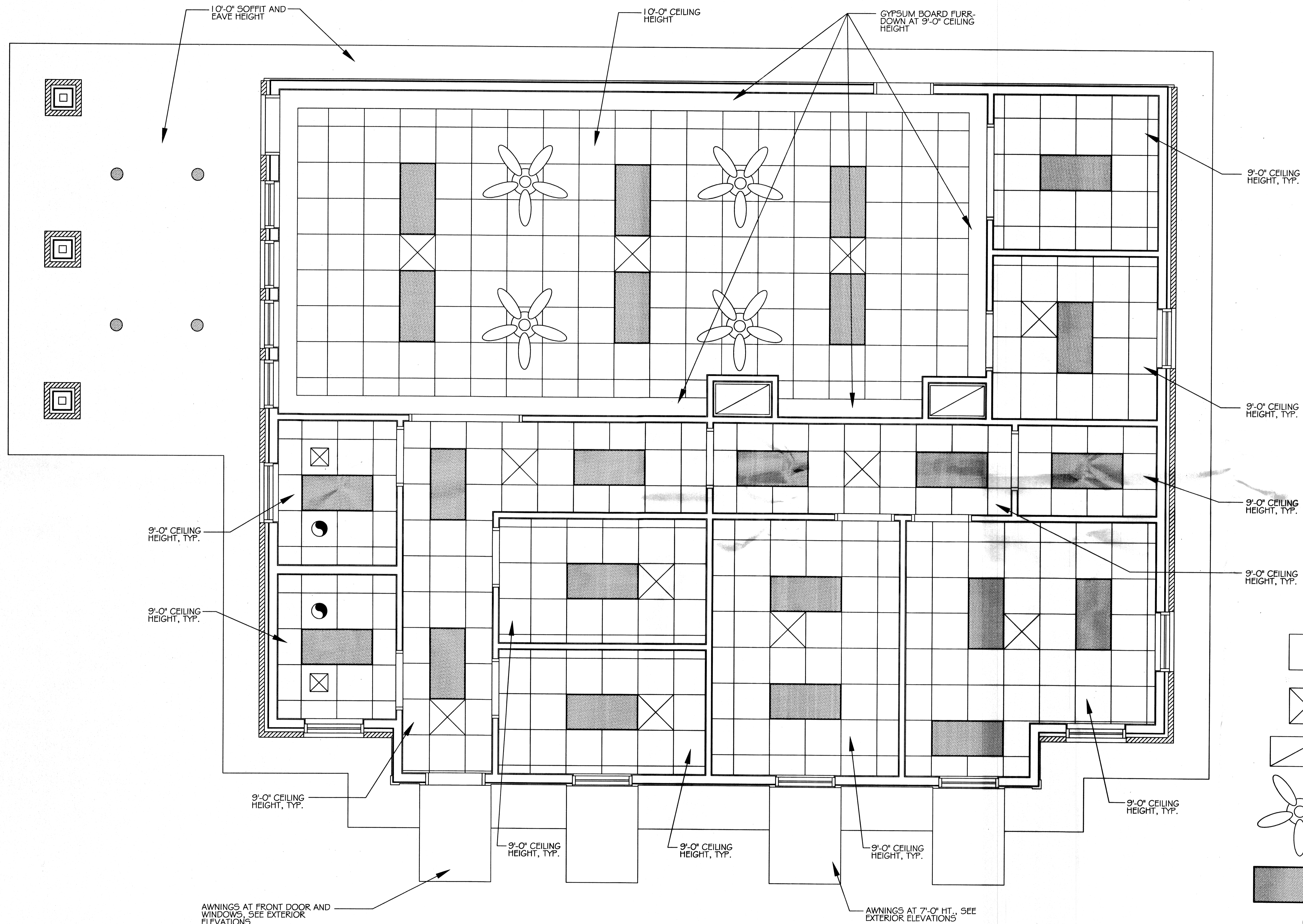
REFLECTED CEILING PLAN SCALE: 3/8" = 1'
