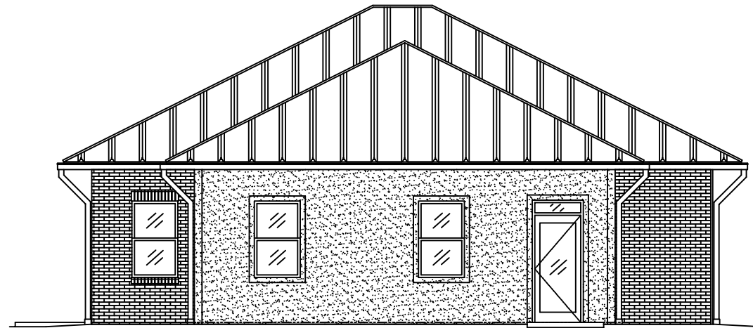
FRONT ELEVATION SCALE: 1/4"=1'
