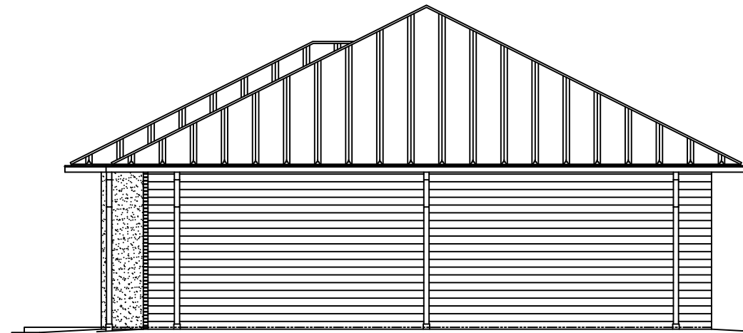
RIGHT SIDE ELEVATION SCALE: 1/4"=1'
