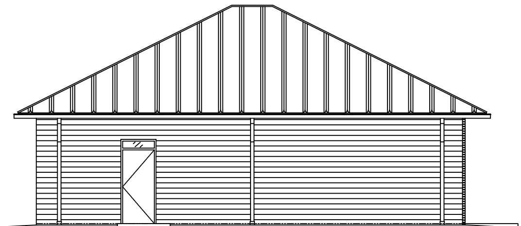
REAR ELEVATION SCALE: 1/4"=1'
