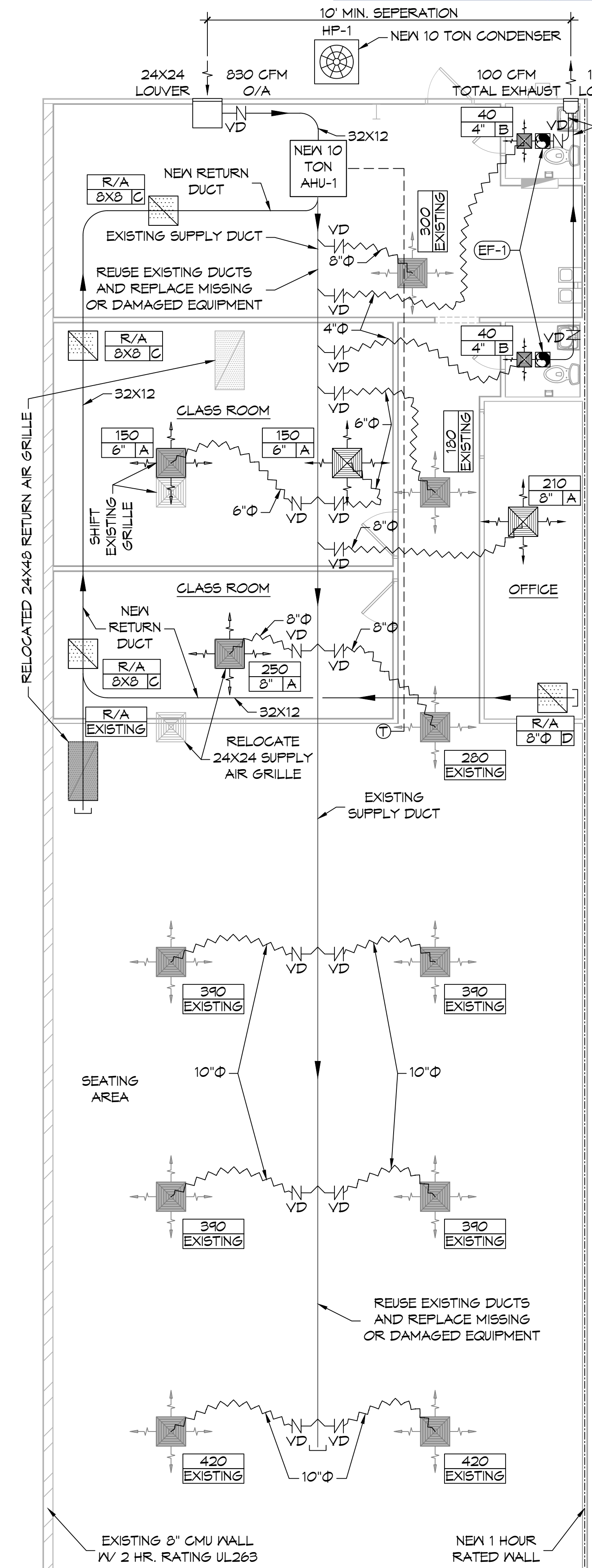
12 MECHANICAL PLAN SCALE: 3/16"=1'-0"
