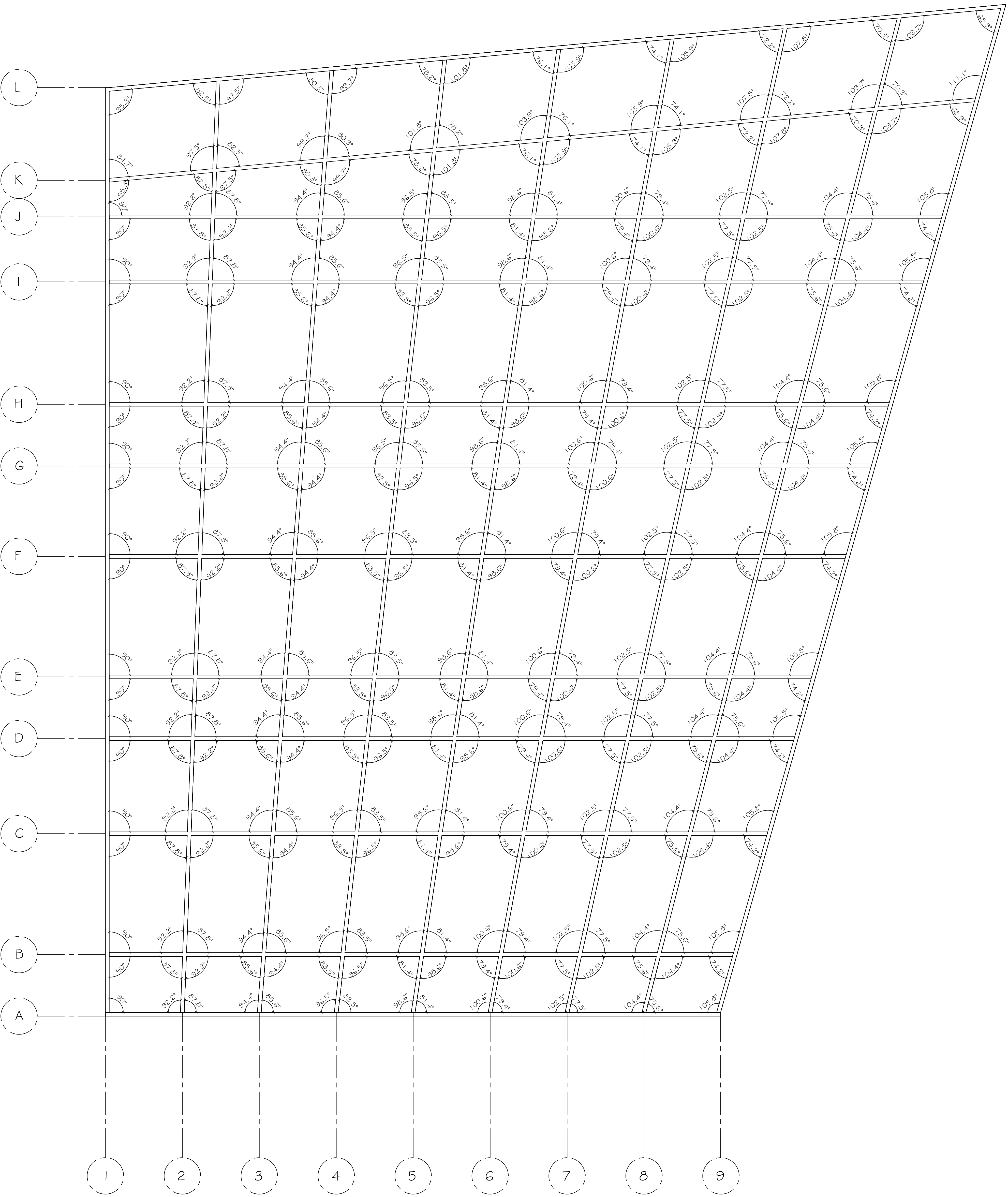
ANGULAR DIMENSIONS
