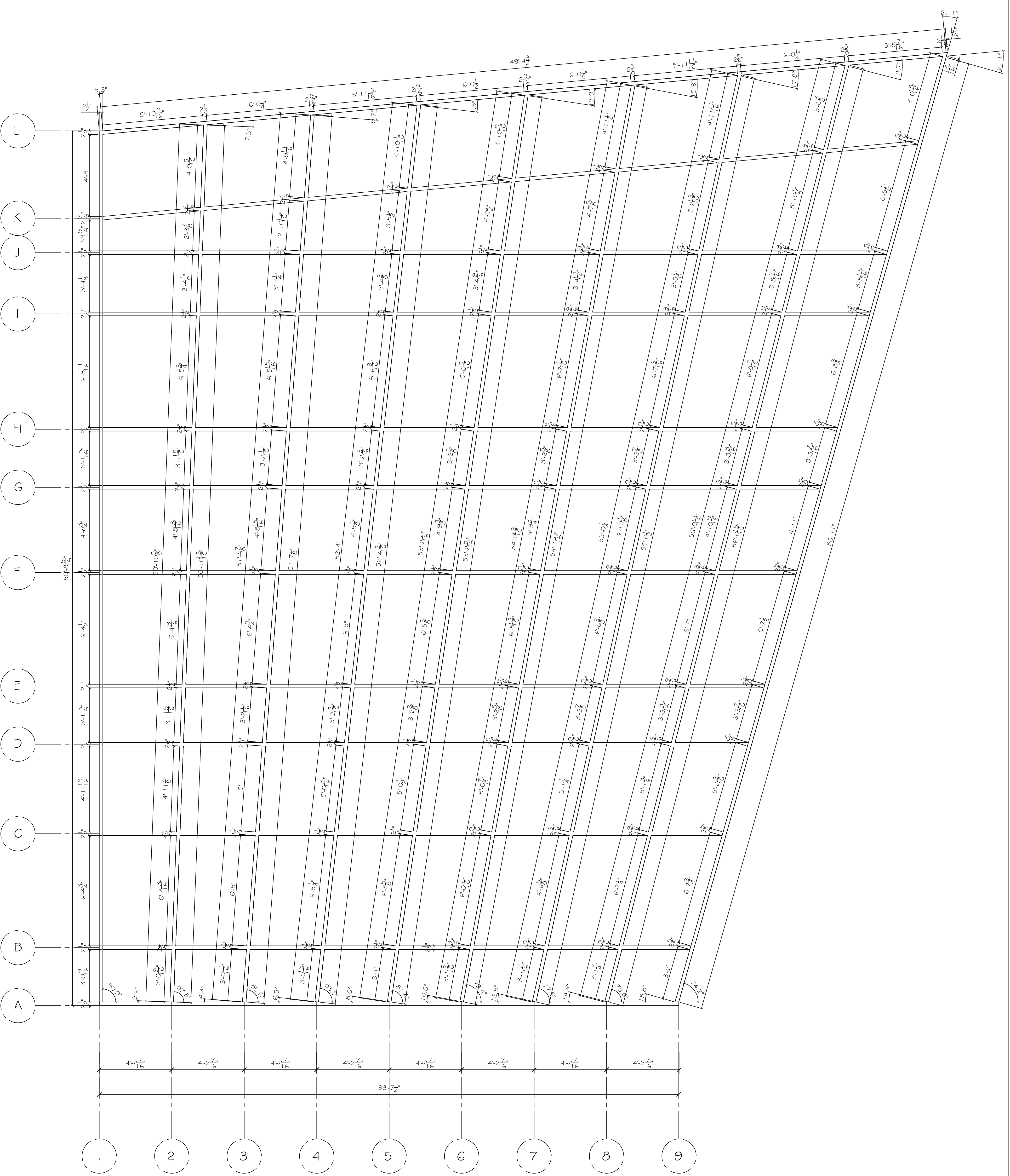
VERTICAL DIMENSIONS
