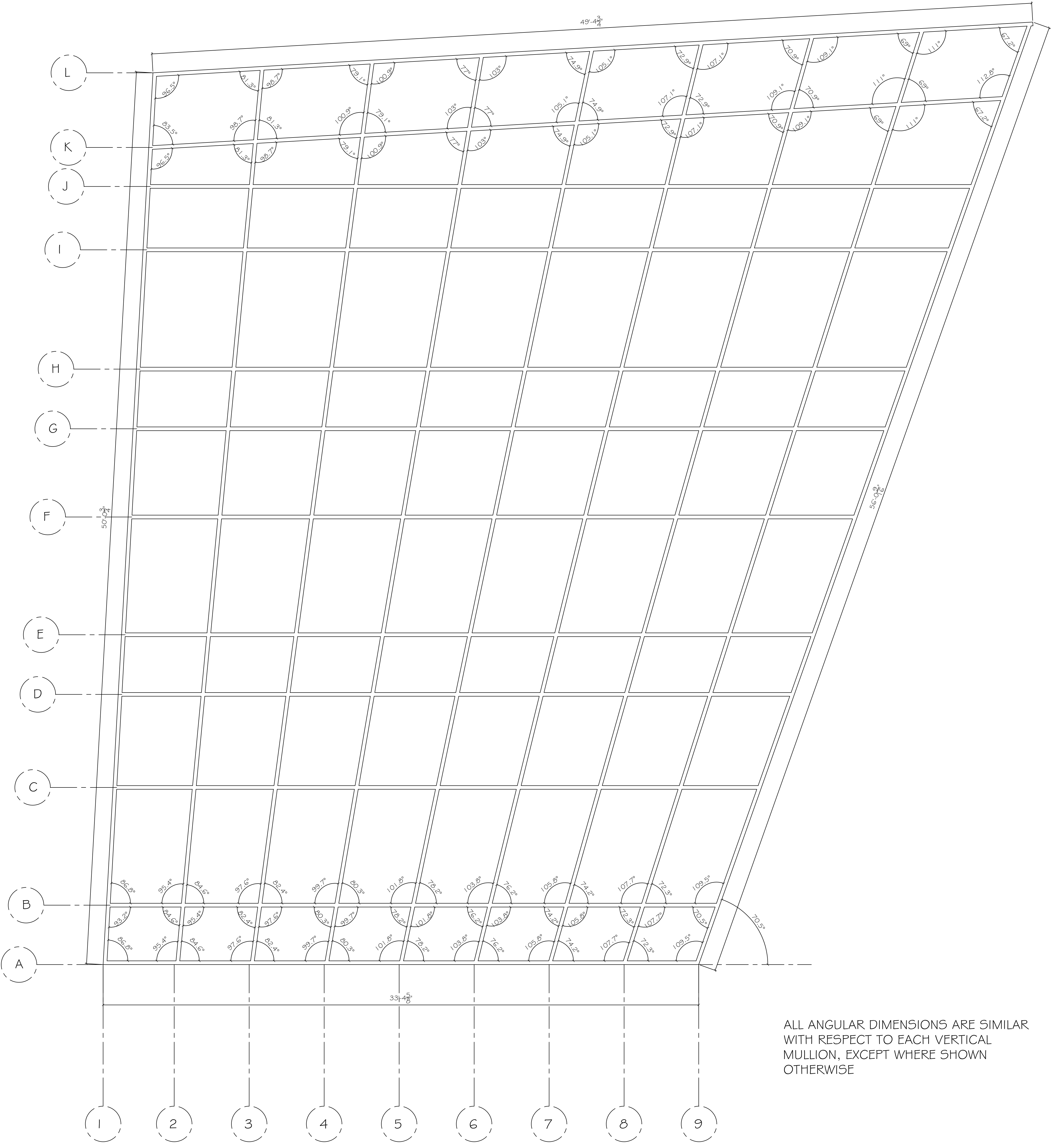
SOUTHWEST GLASS WALL DIMENSIONS SCALE 3/8" = 1'-0"
