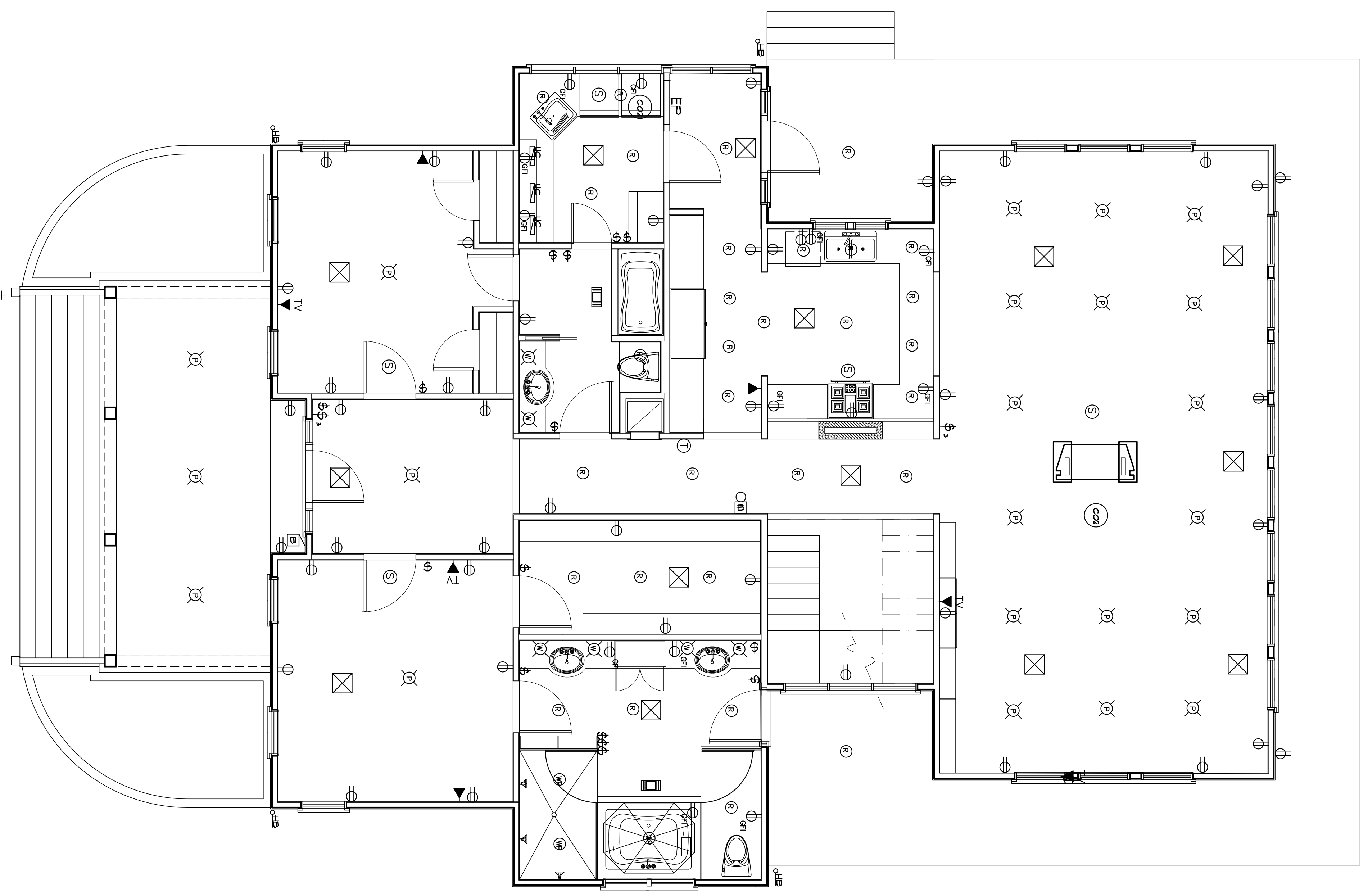
First Floor HVAC Plan Scale: 1/4" = 1'-0"
