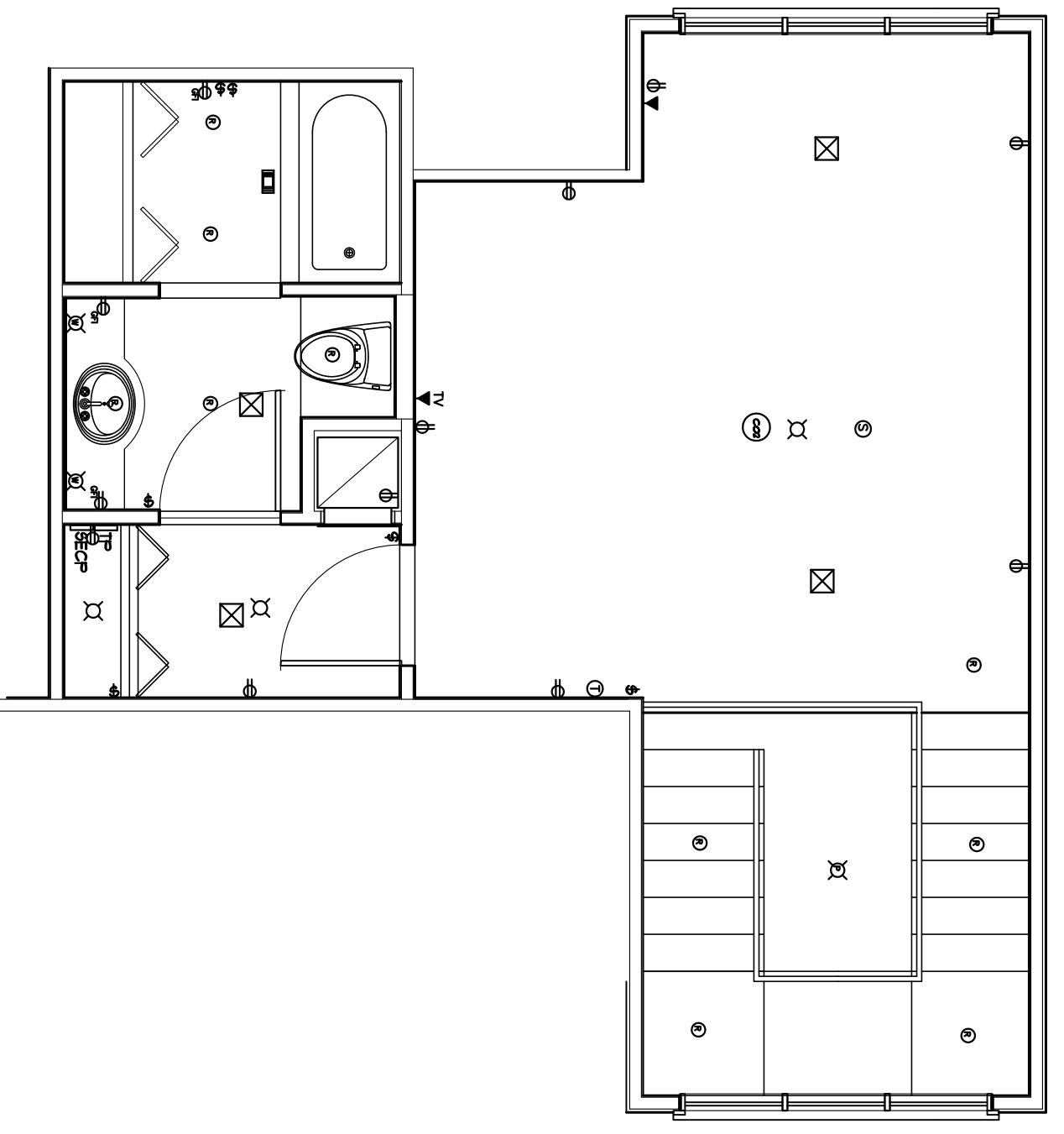
Second Floor HVAC Plan Scale: 1/4" = 1'-0"
