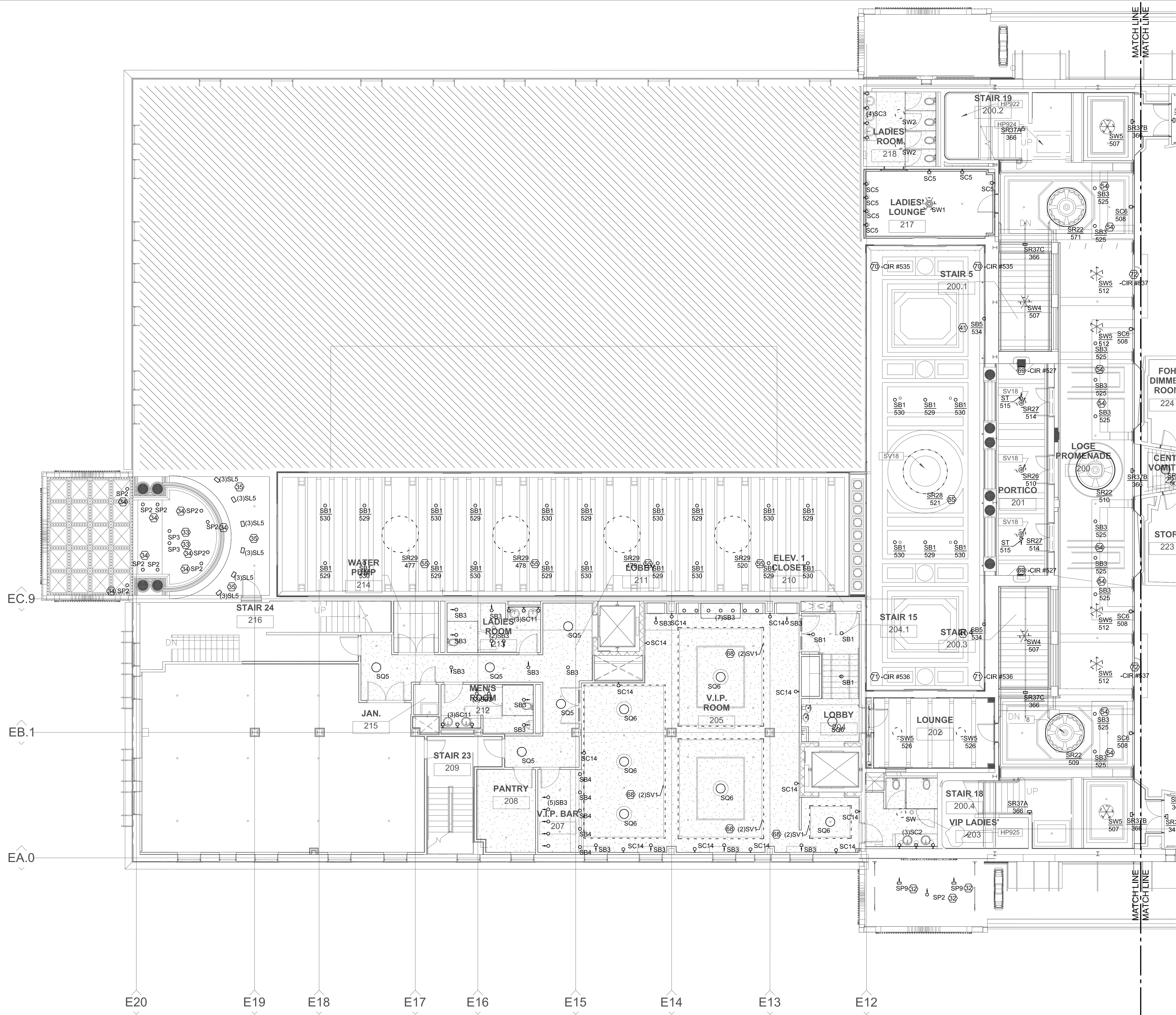
1 ARCHITECTURAL PARTIAL LIGHTING PLAN - ARCADE - LOGE LEVEL AL-1.03 / SCALE: 1/8" = 1'-0"
