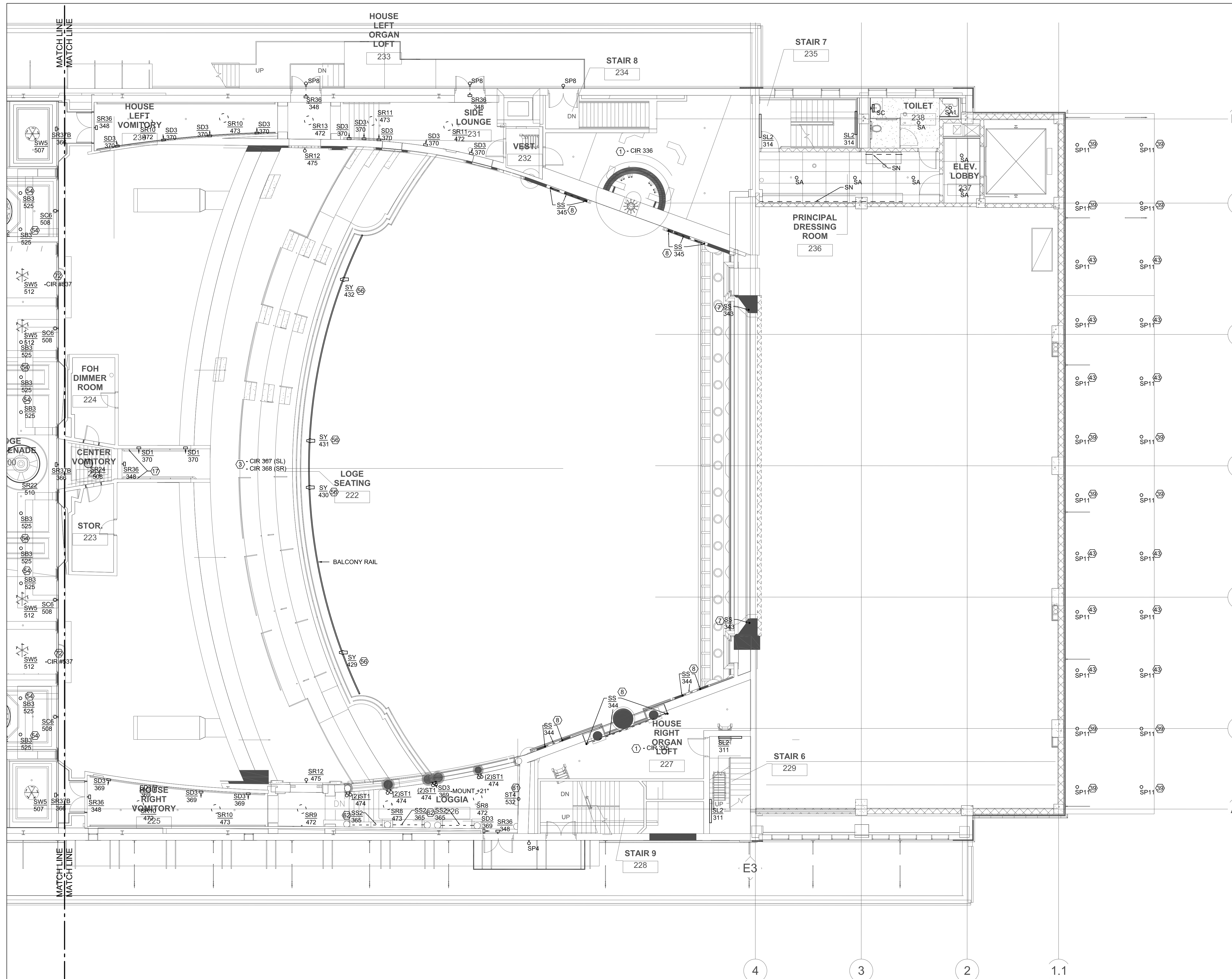
1 ARCHITECTURAL LIGHTING PLAN - LOGE LEVEL AL-1.04 / SCALE: 1/8" = 1'-0"
