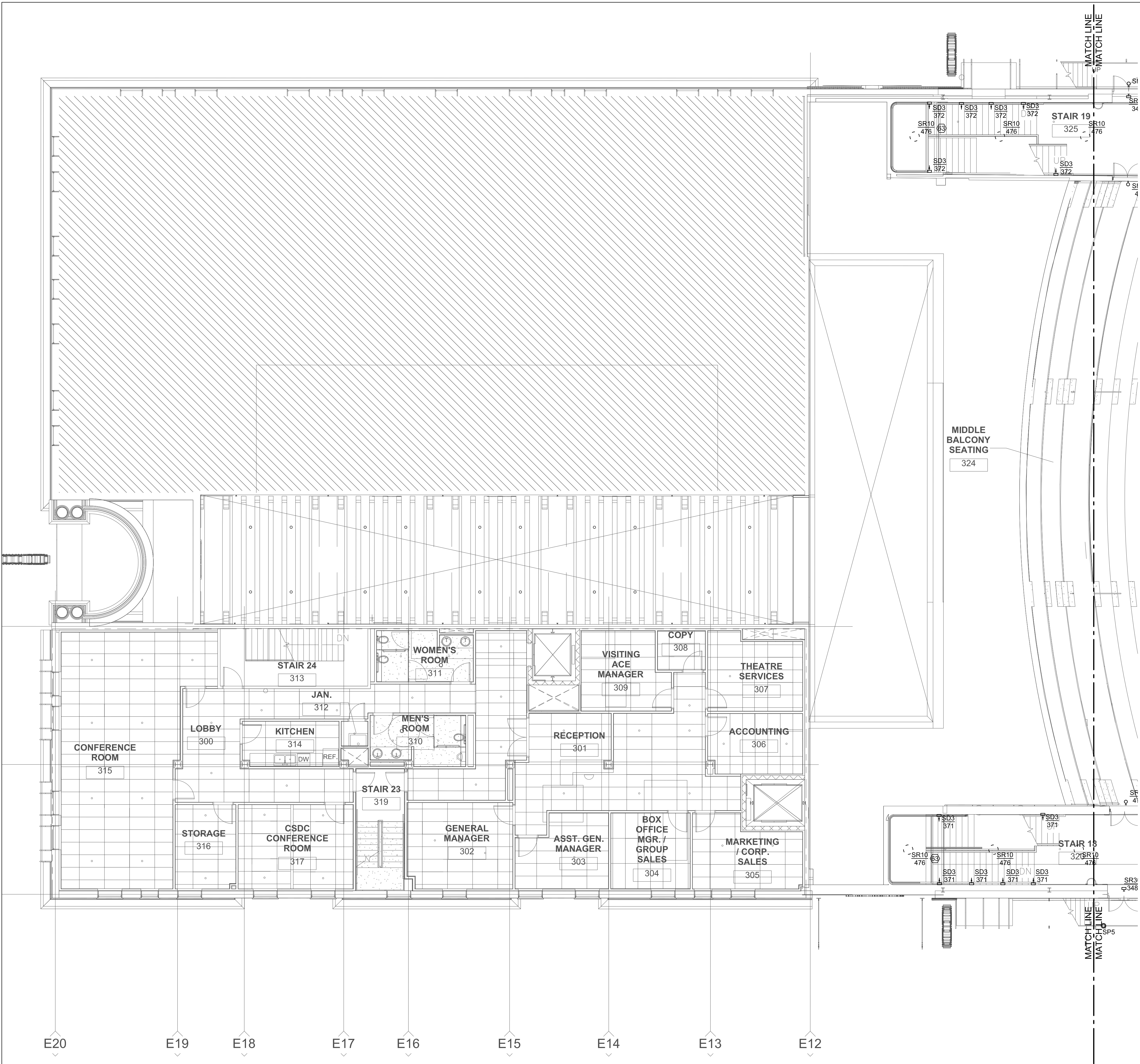
1 ARCHITECTURAL LIGHTING PLAN - ARCADE - MIDDLE BALCONY LEVEL AL-1.06 / SCALE: 1/8" = 1'-0"
