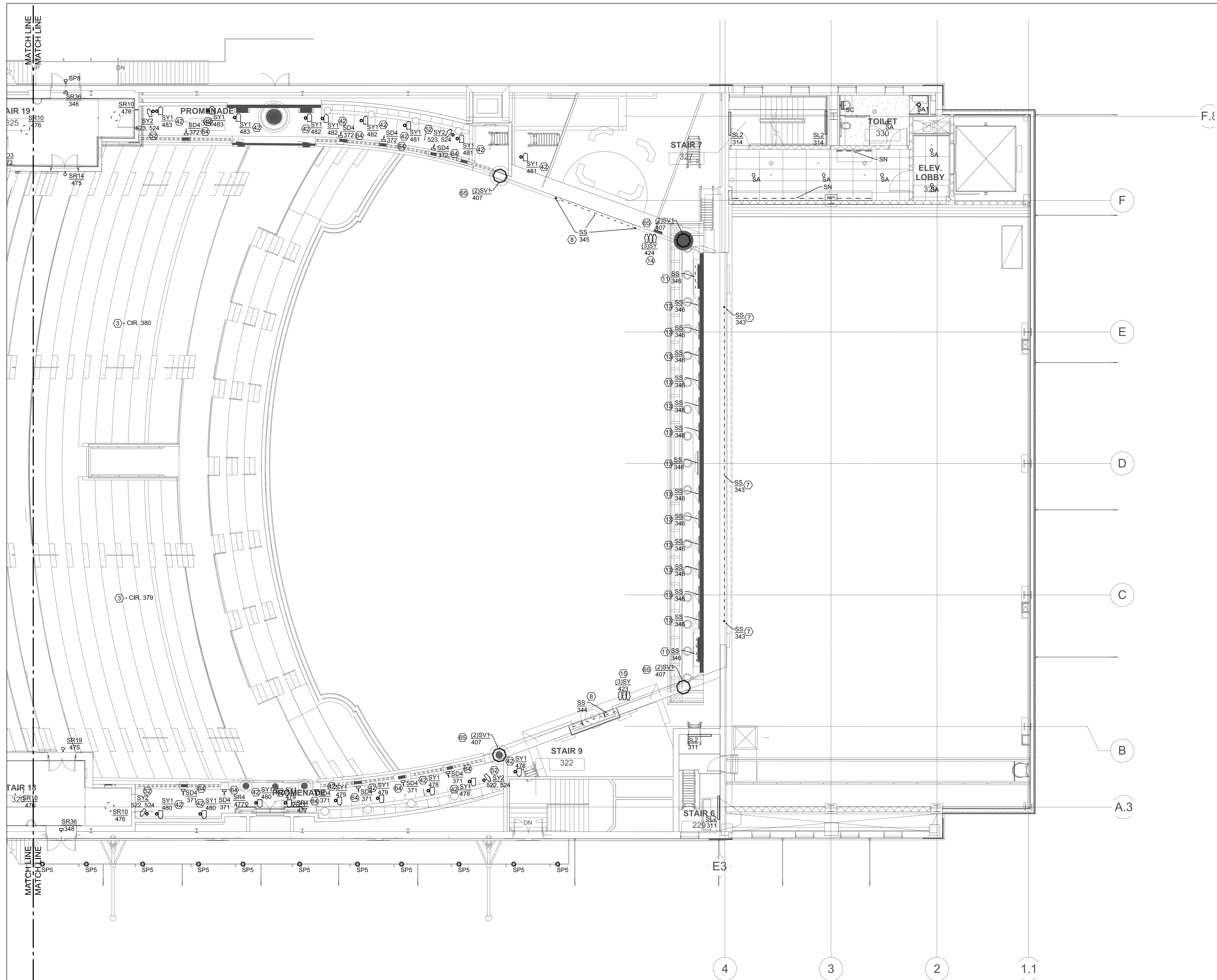
1 ARCHITECTURAL LIGHTING PLAN - MIDDLE BALCONY LEVEL AL-1.07 SCALE: 1/8" = 1'-0"
