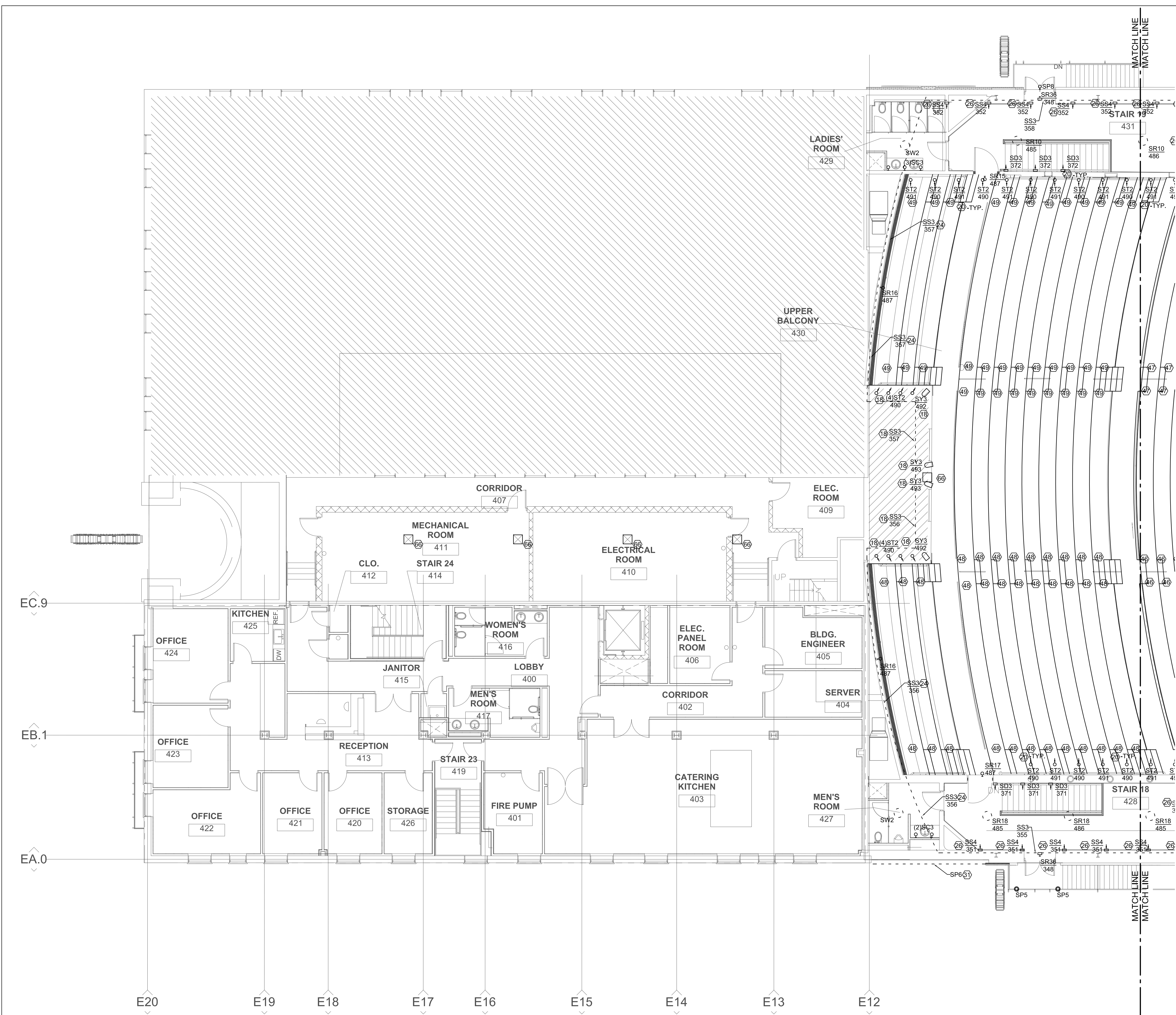
1 ARCHITECTURAL LIGHTING PLAN - ARCADE - BALCONY LEVEL AL-1.08 / SCALE: 1/8" = 1'-0"
