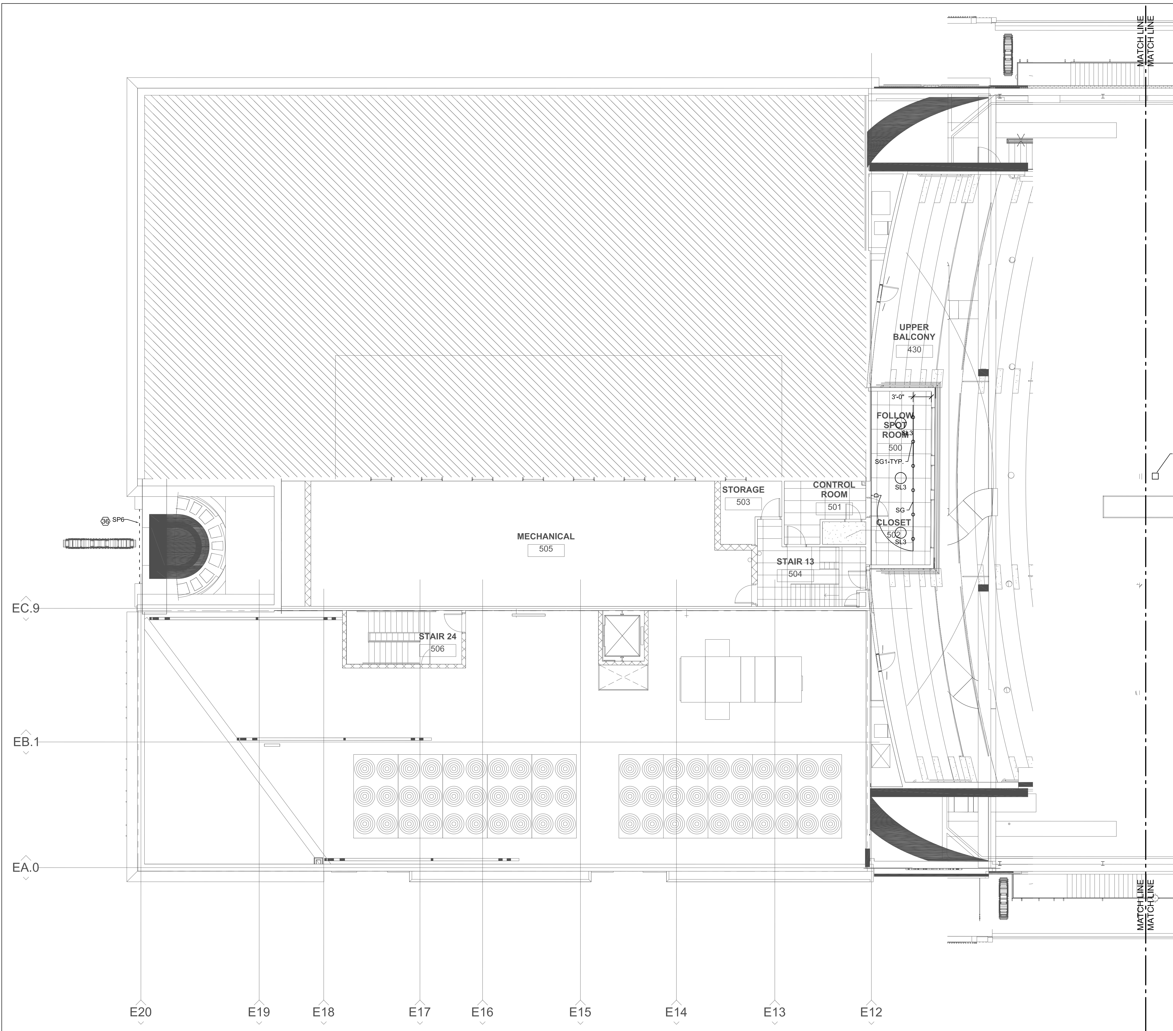
1 ARCHITECTURAL LIGHTING PLAN - CONTROL LEVEL AL-1.10 / SCALE: 1/8" = 1'-0"
