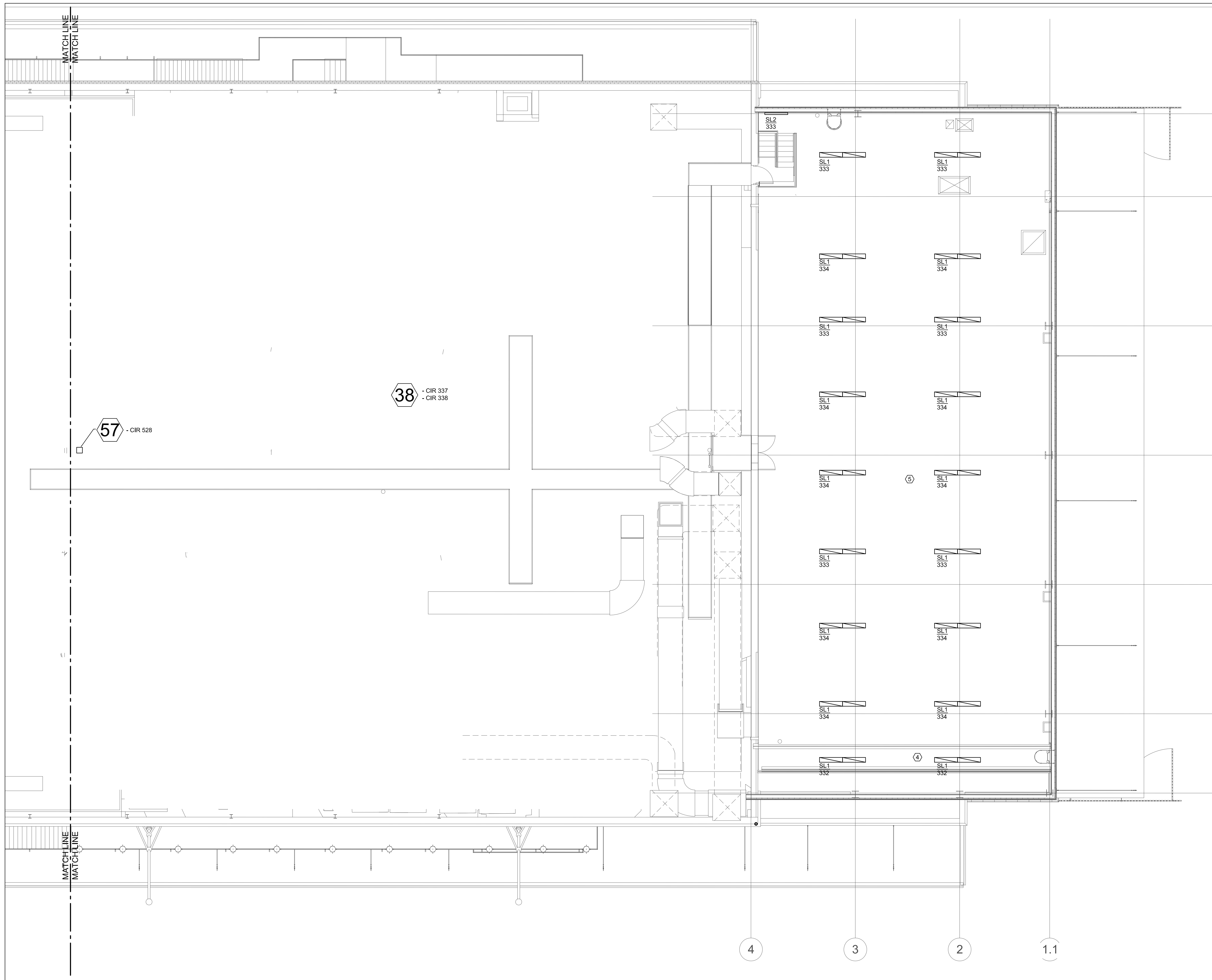
1 ARCHITECTURAL LIGHTING PLAN - GRID IRON LEVEL AL-1.11 SCALE: 1/8" = 1'-0"
