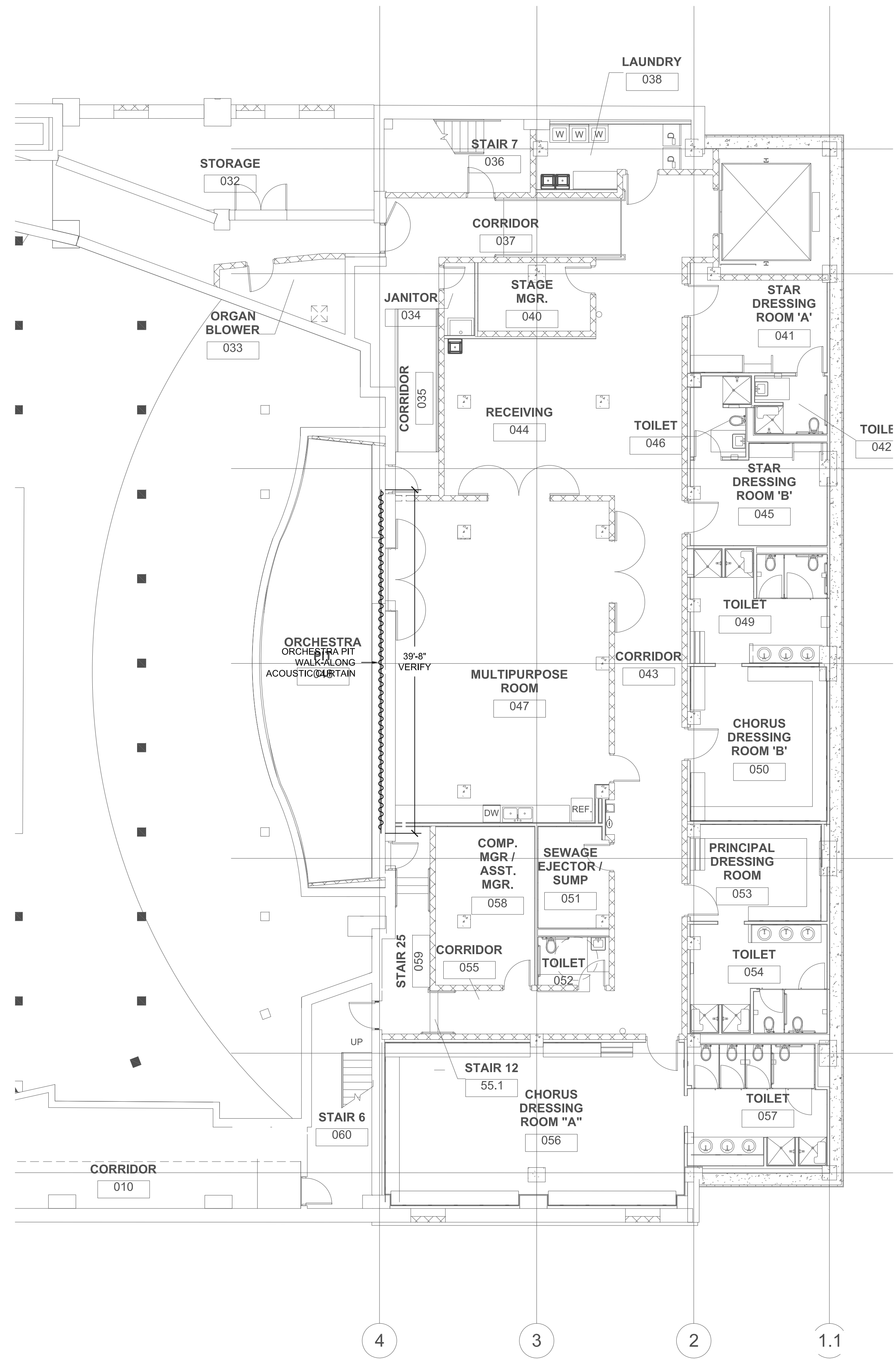
1 THEATRE RIGGING PLAN - BASEMENT LEVEL TR-1.02 SCALE: 1/8" = 1'-0"
