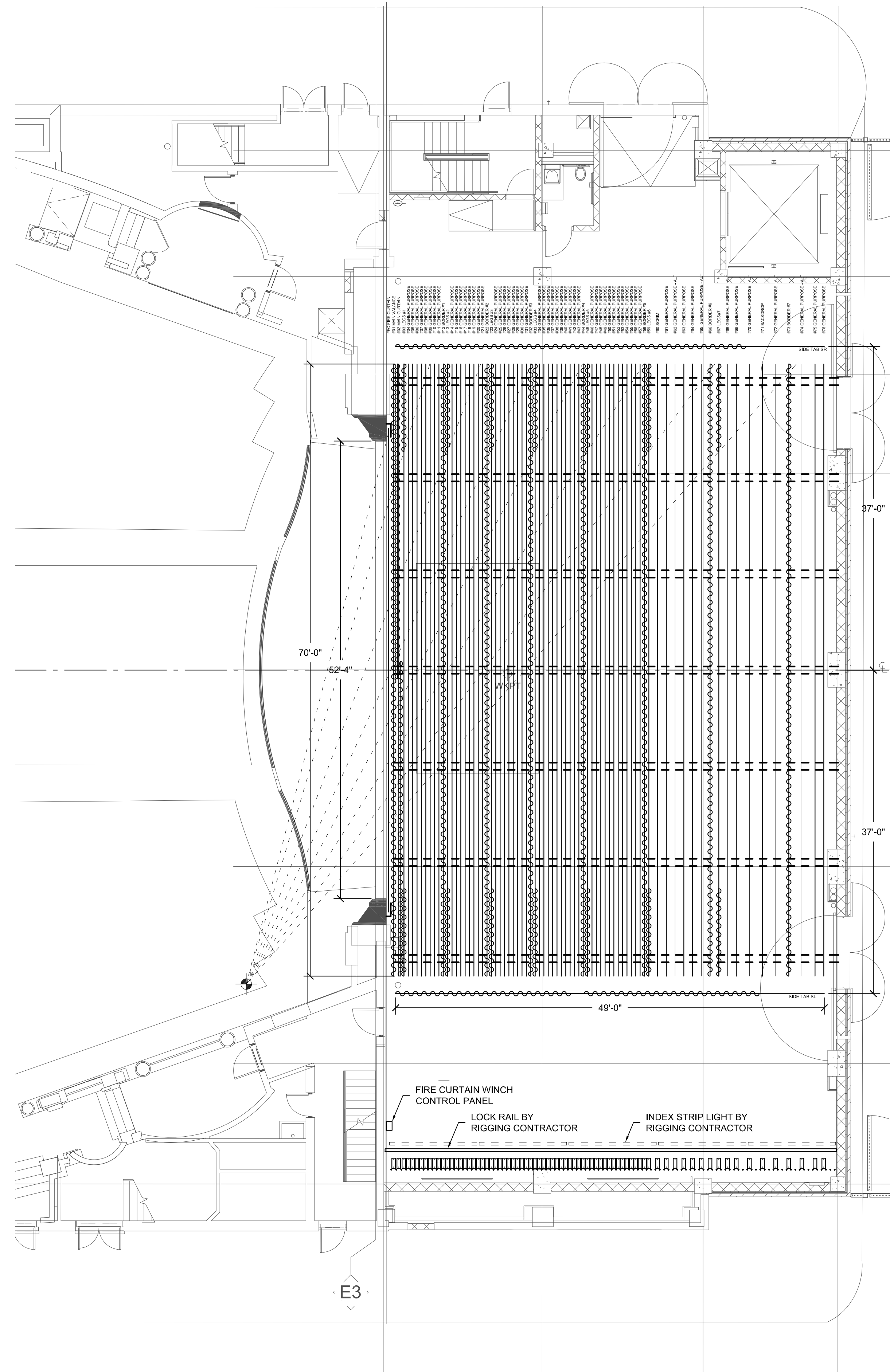
2 THEATRE RIGGING PLAN - ORCHESTRA LEVEL TR-1.02 SCALE: 1/8" = 1'-0"
