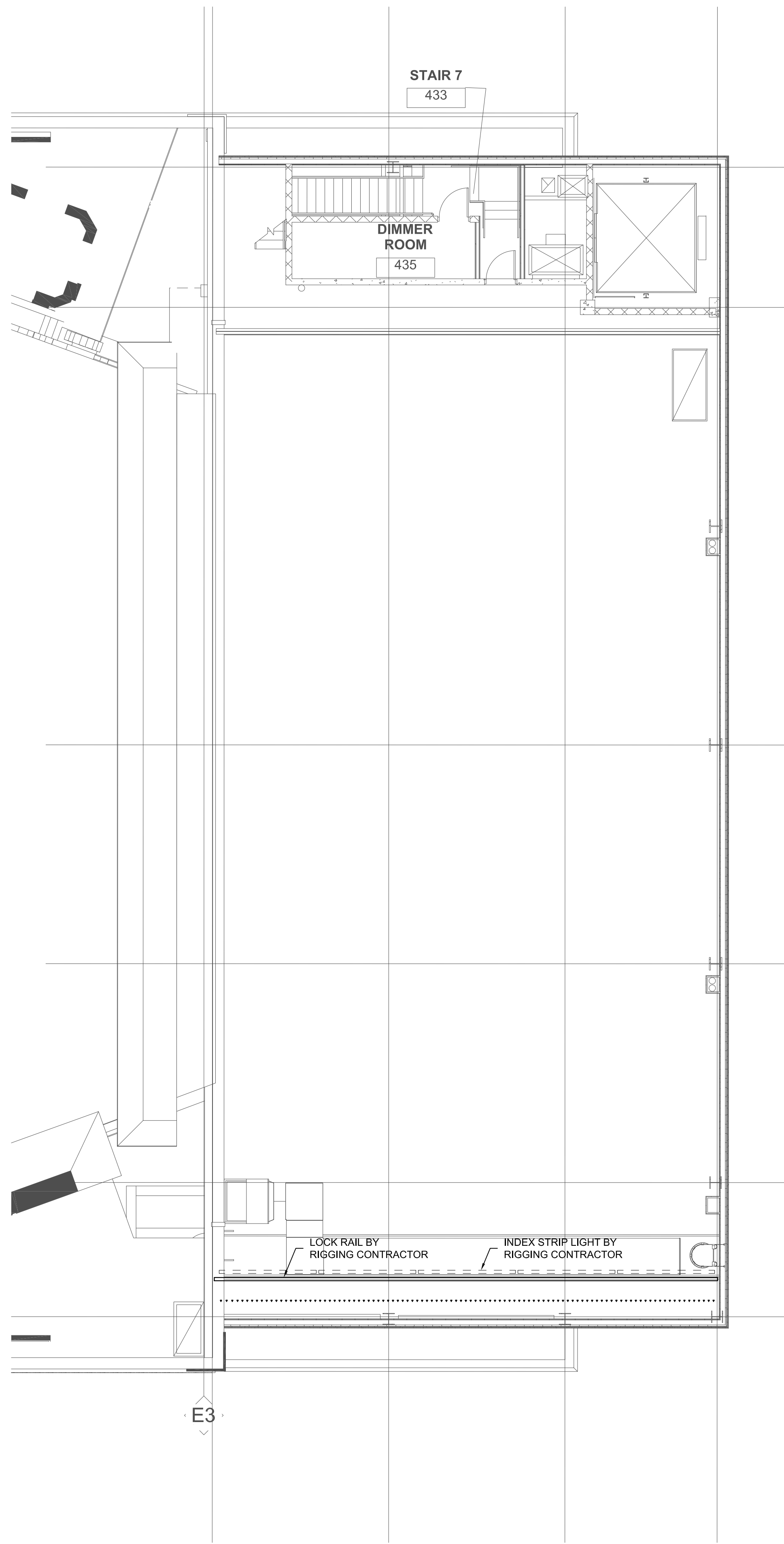
1 THEATRE RIGGING PLAN - PINRAIL GALLERY LEVEL TR-1.11 SCALE: 1/8" = 1'-0"
