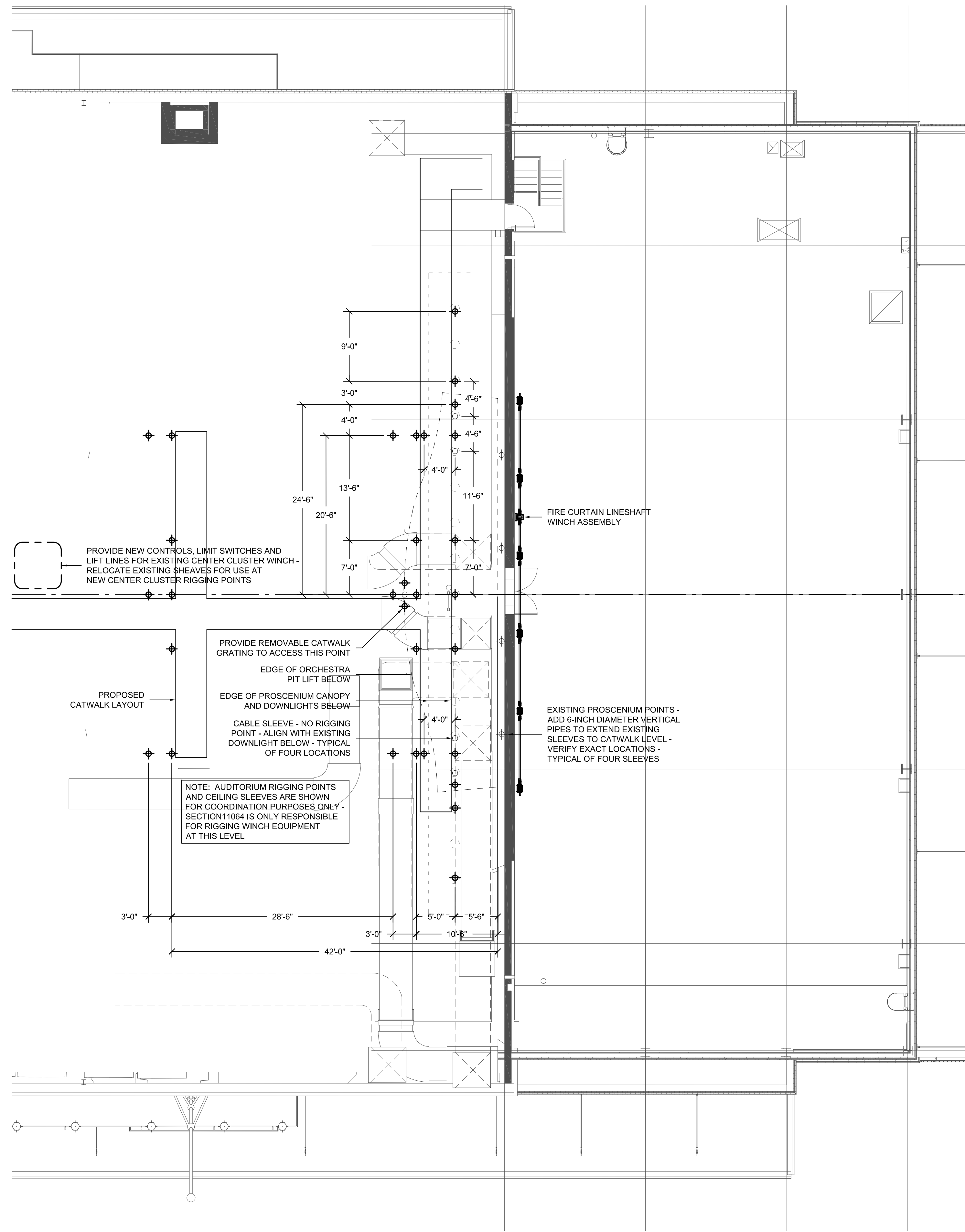
2 THEATRE RIGGING PLAN - ATTIC / GRIDIRON LEVEL TR-1.11 SCALE: 1/8" = 1'-0"
