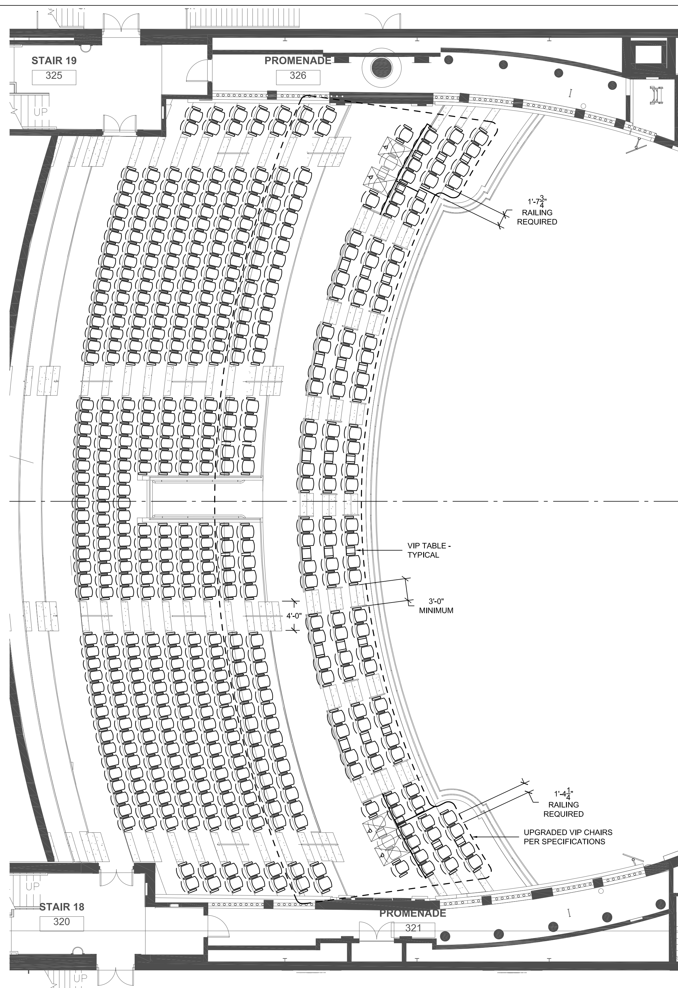
2 THEATRE SEATING PLAN - LOGE AND MIDDLE BALCONY LEVEL
