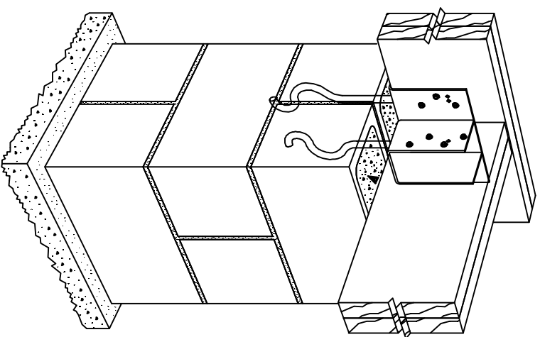
TYPICAL CCTQM INSTALLATION
