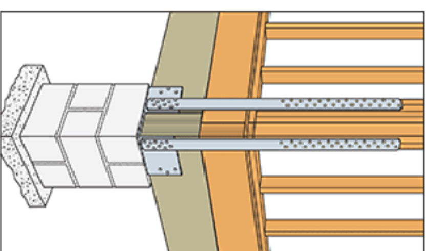
TYPICAL ECCLQM INSTALLATION
