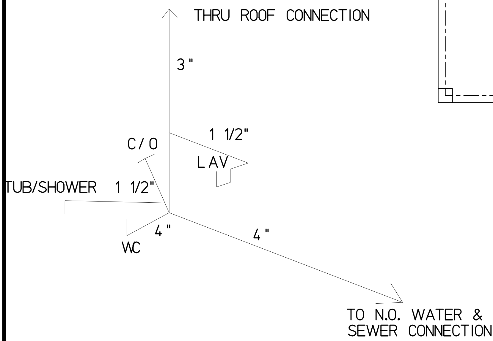
TYPICAL BATHROOM PLUMBING RISER PLAN NT.5.
