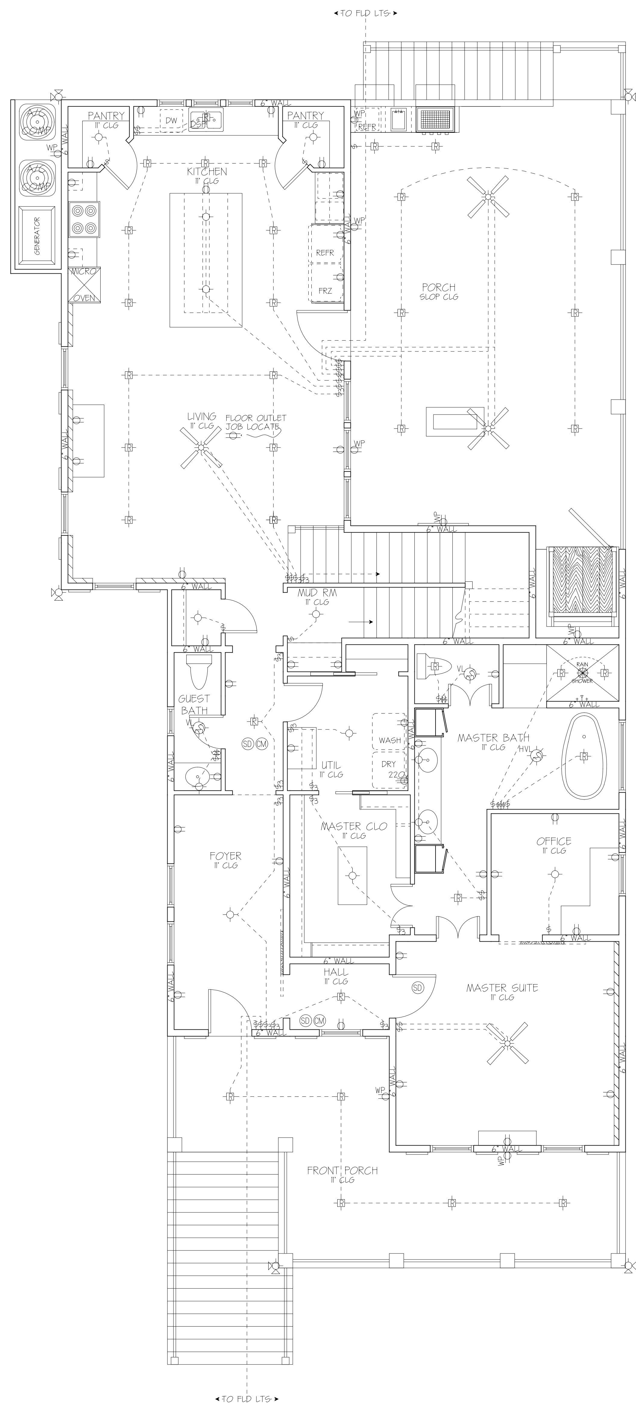
1ST LEVEL ELECTRICAL PLAN SCALE 1/4"=1'-0"
