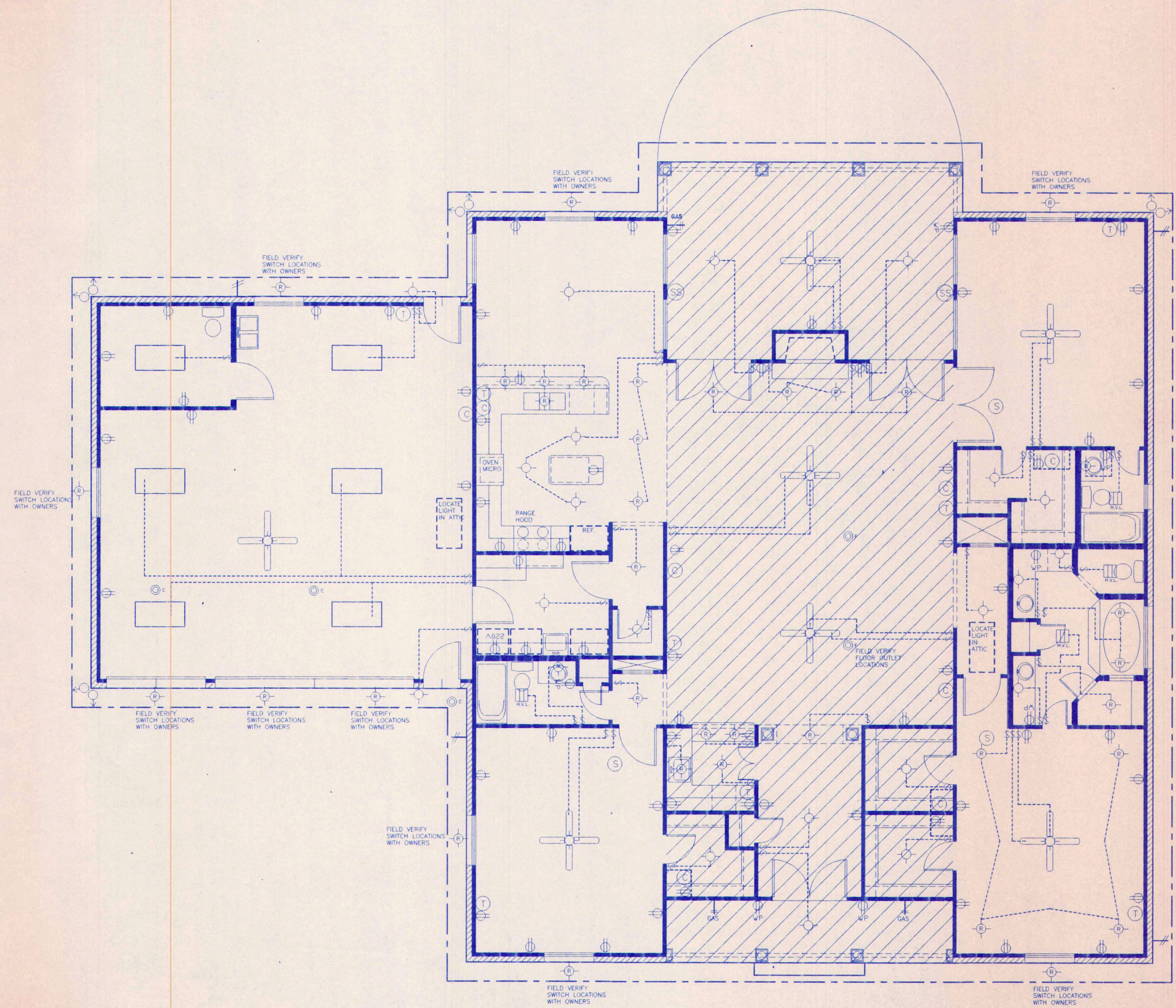
ELECTRICAL FLOOR PLAN SCALE : 1/4" = 1'-0"
