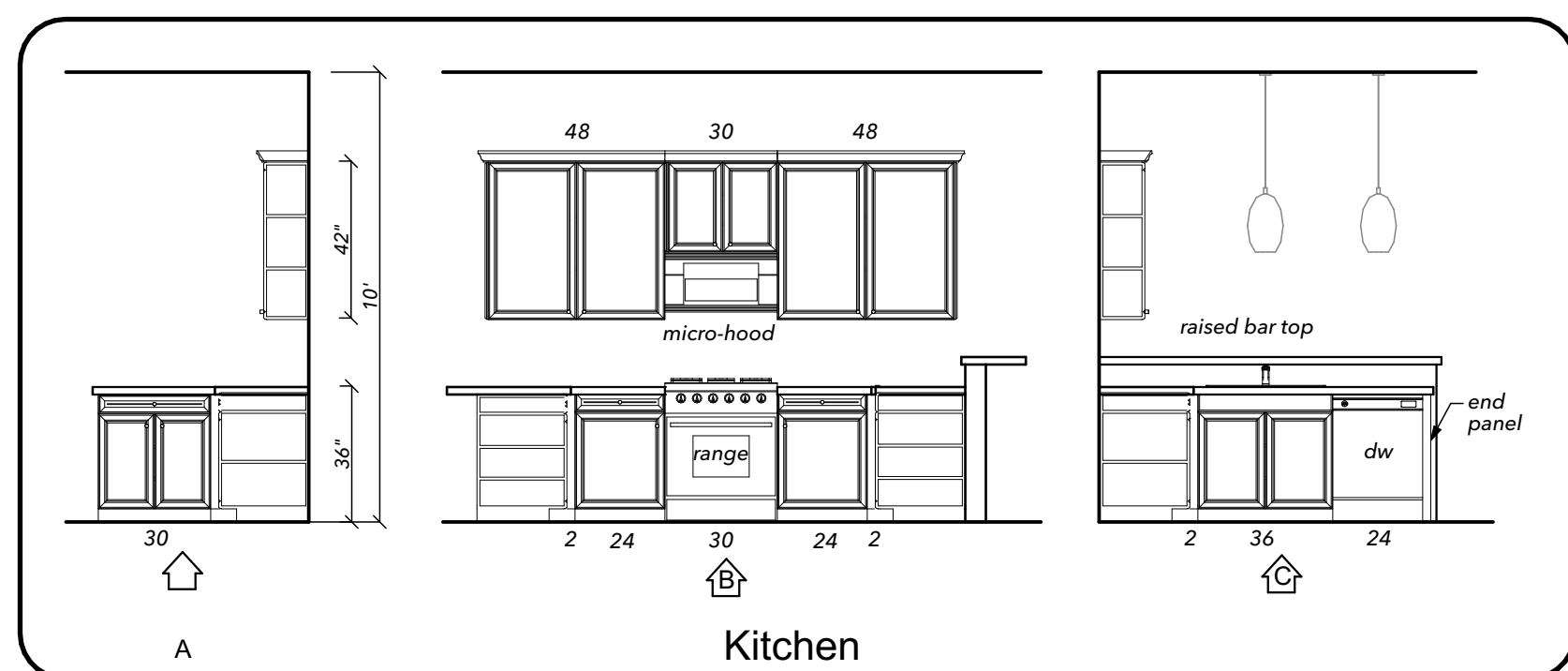
Cabinet Details Scale: 1/4" = 1'-0"
