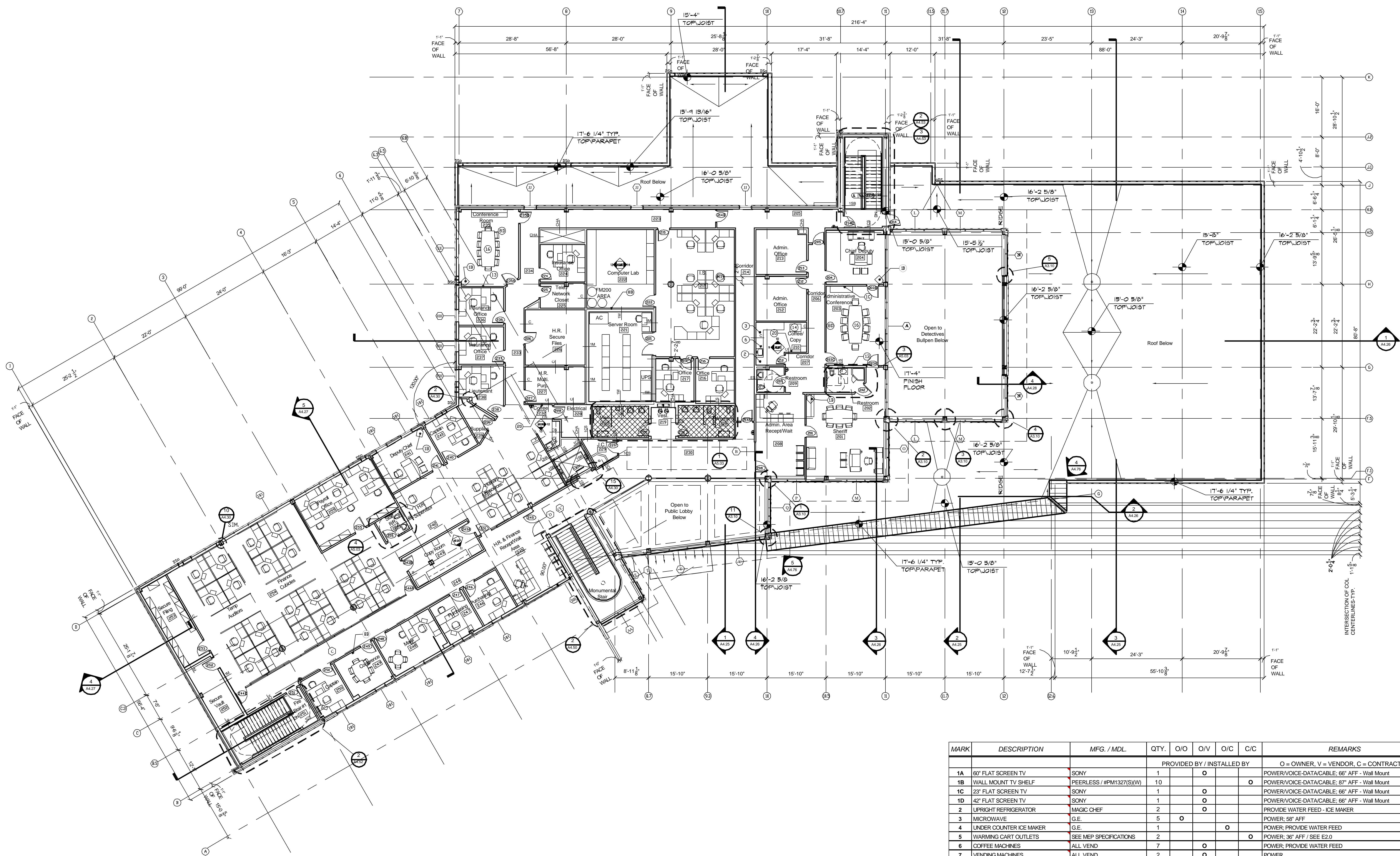
1 2ND FLOOR REFERENCE PLAN A2.02 3/32"=1'-0"
