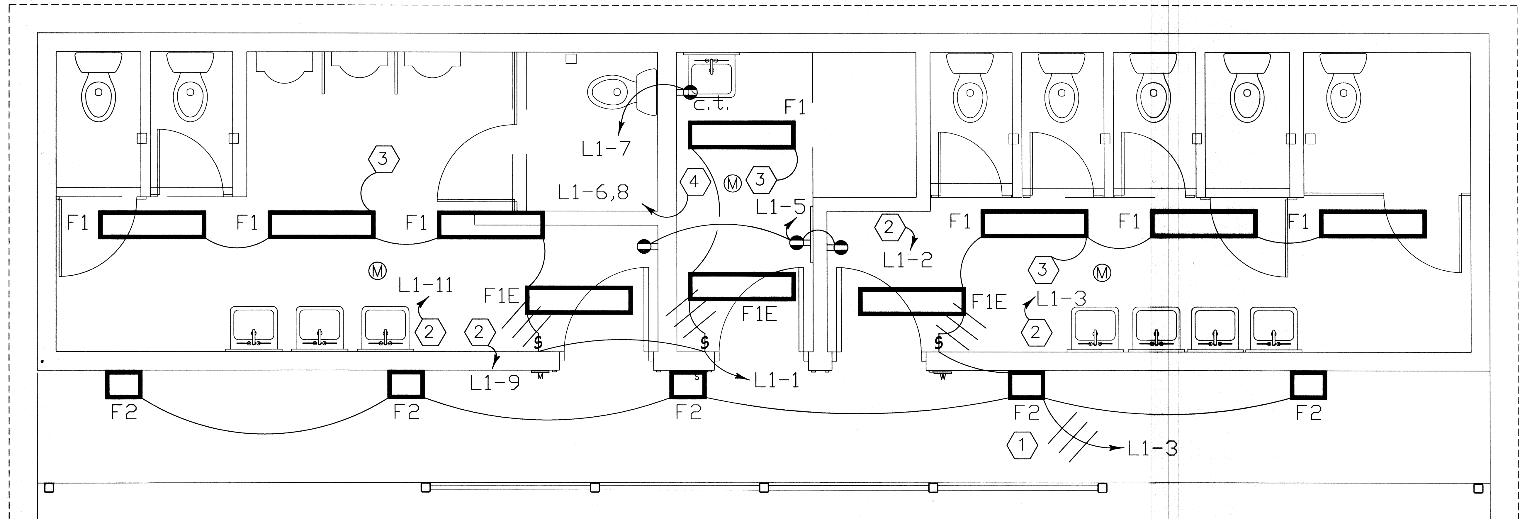
FLOOR PLAN 1/4" = 1'
