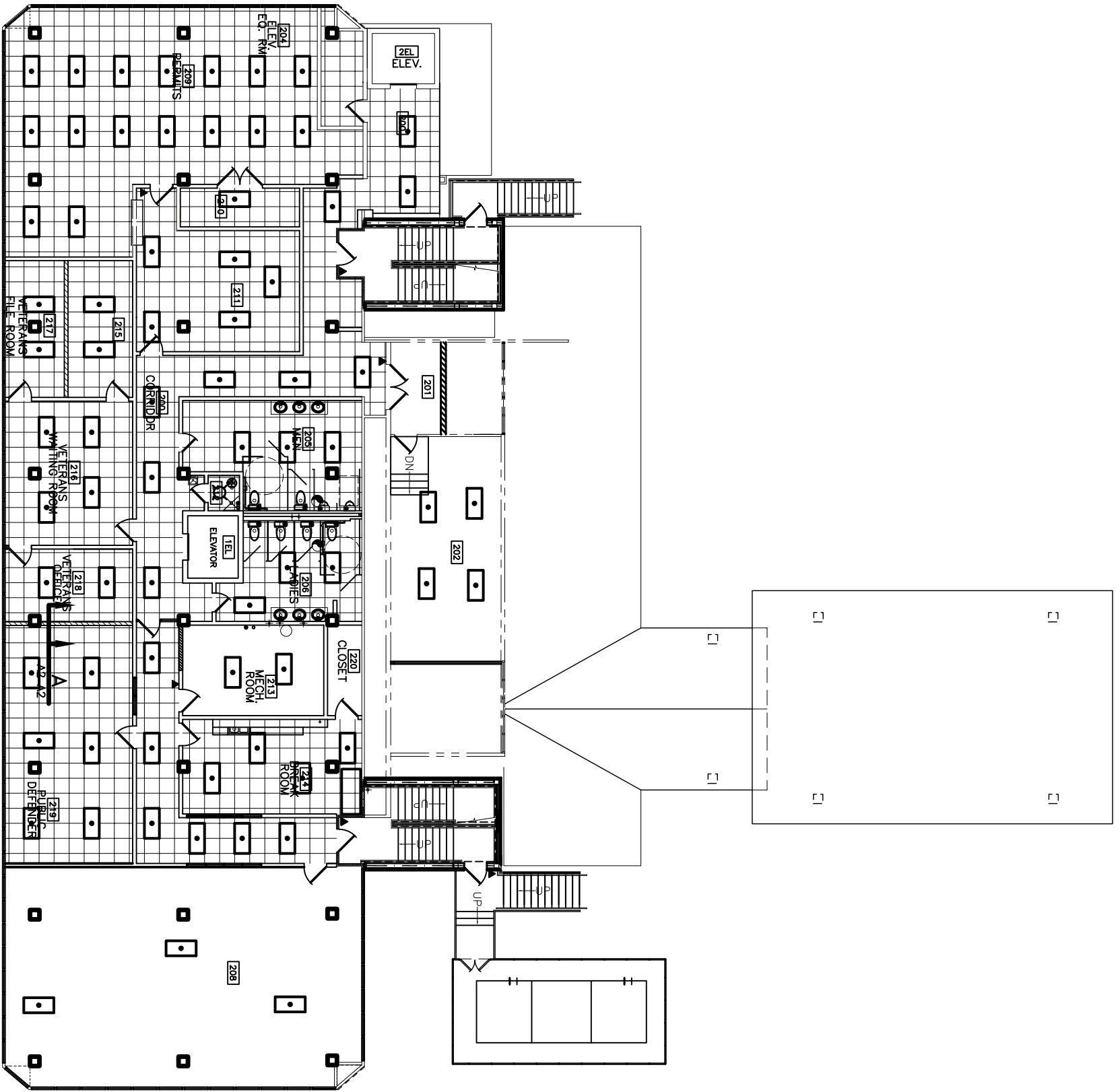
SECOND FLOOR REFLECTED CEILING PLAN SCALE: 1/8" = 1'-0"
