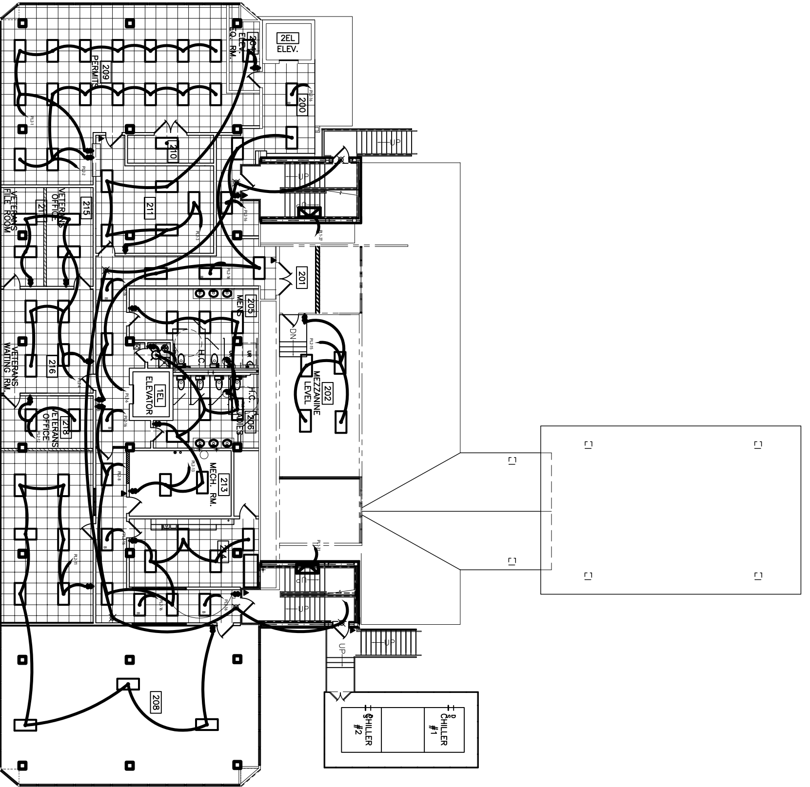
SECOND FLOOR LIGHTING PLAN SCALE: 1/8" = 1'-0"
