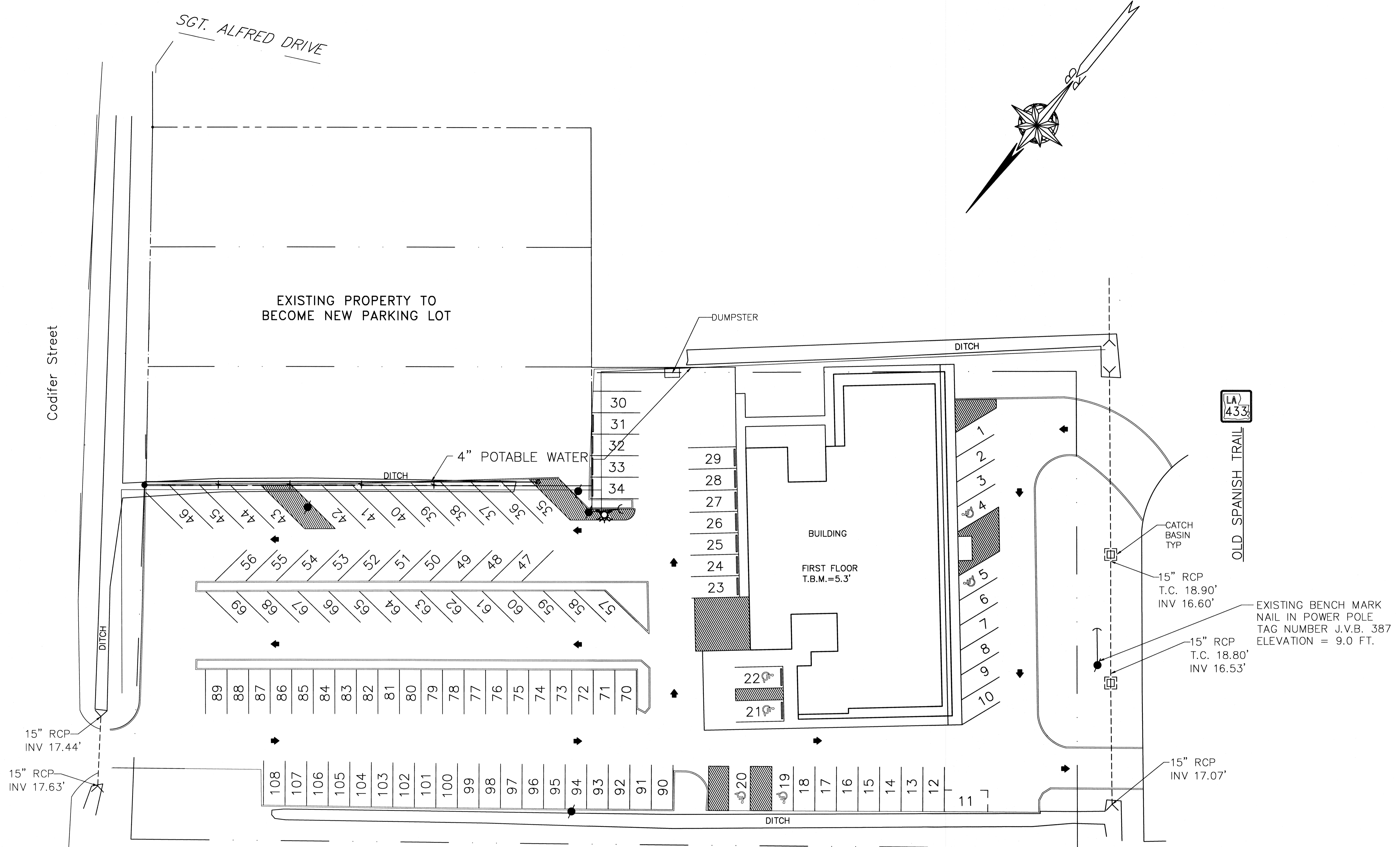
EXISTING SITE PLAN SCALE: 1"=20'-0"
