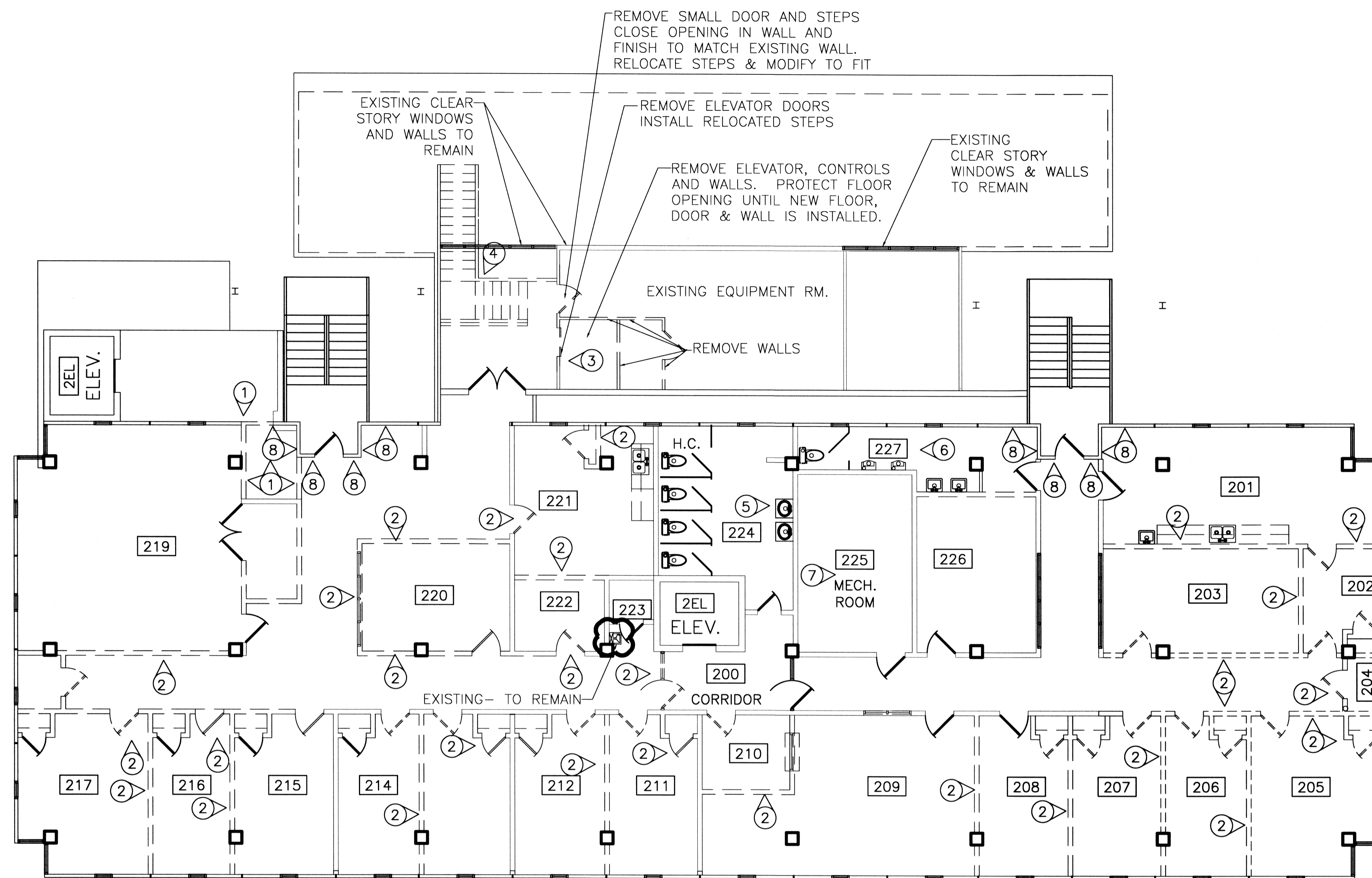
2ND FLOOR DEMOLITION PLAN SCALE: 1/8" = 1'-0"
