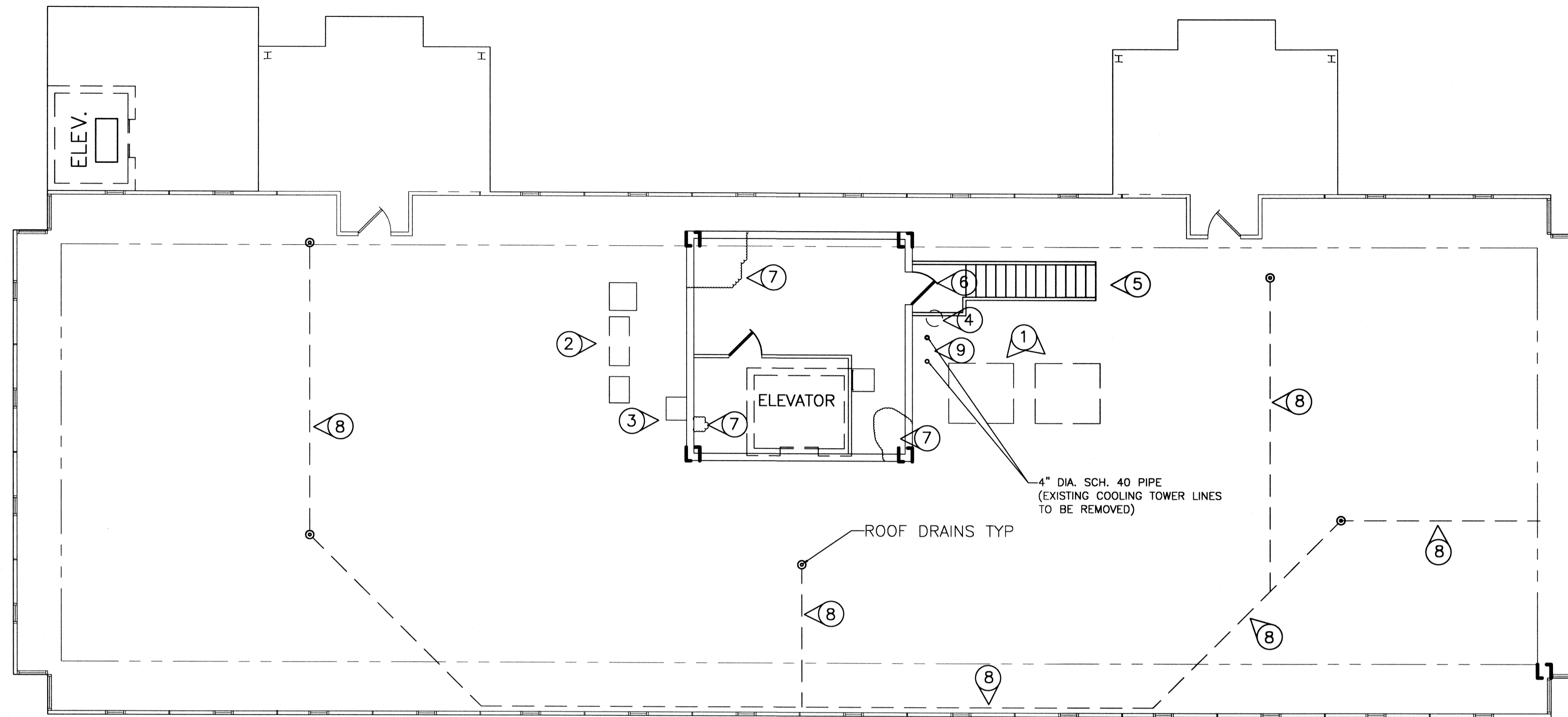
ROOF DEMOLITION PLAN SCALE: 1/8" = 1'-0"
