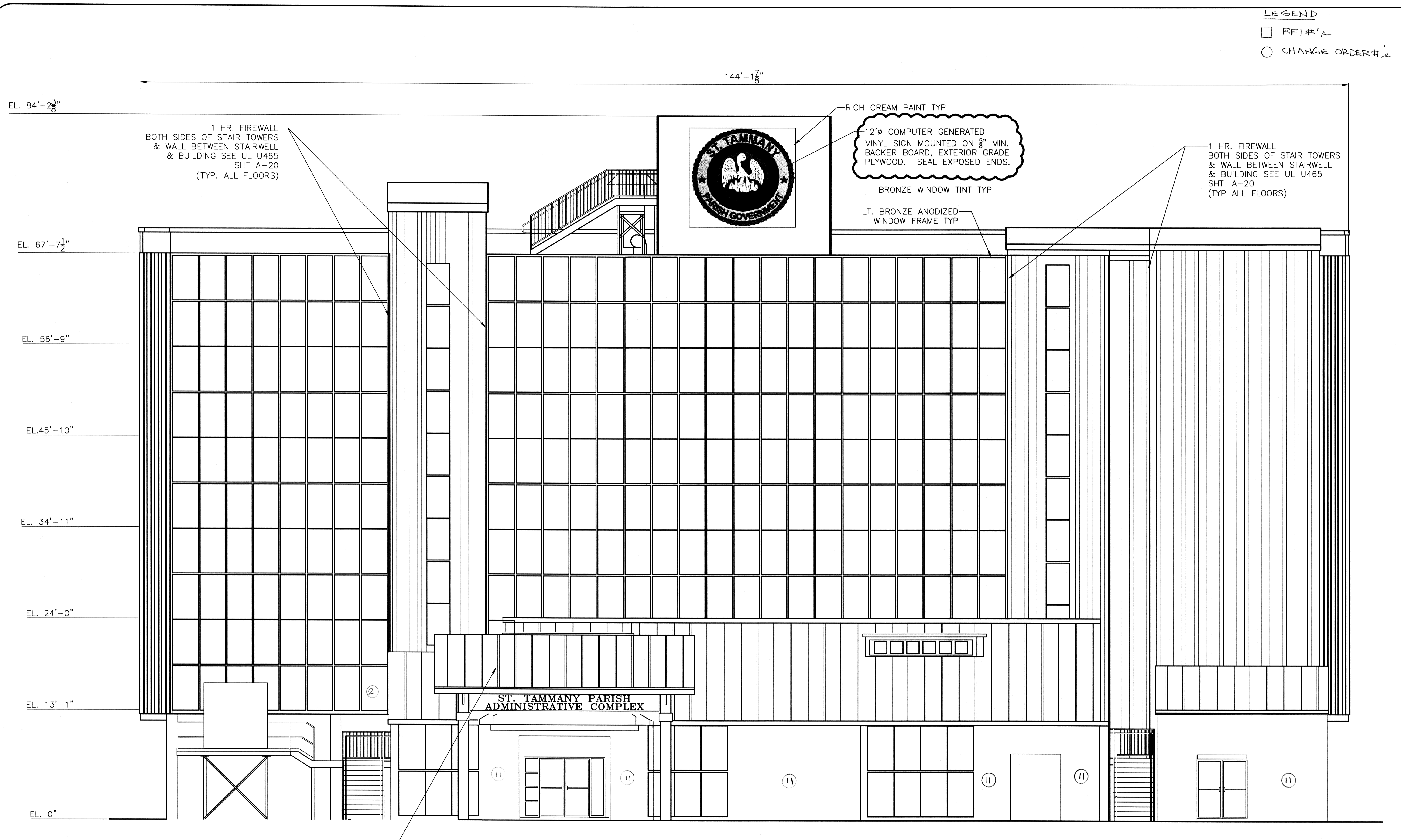
NORTH ELEVATION SCALE: 3/16" = 1'-0"
