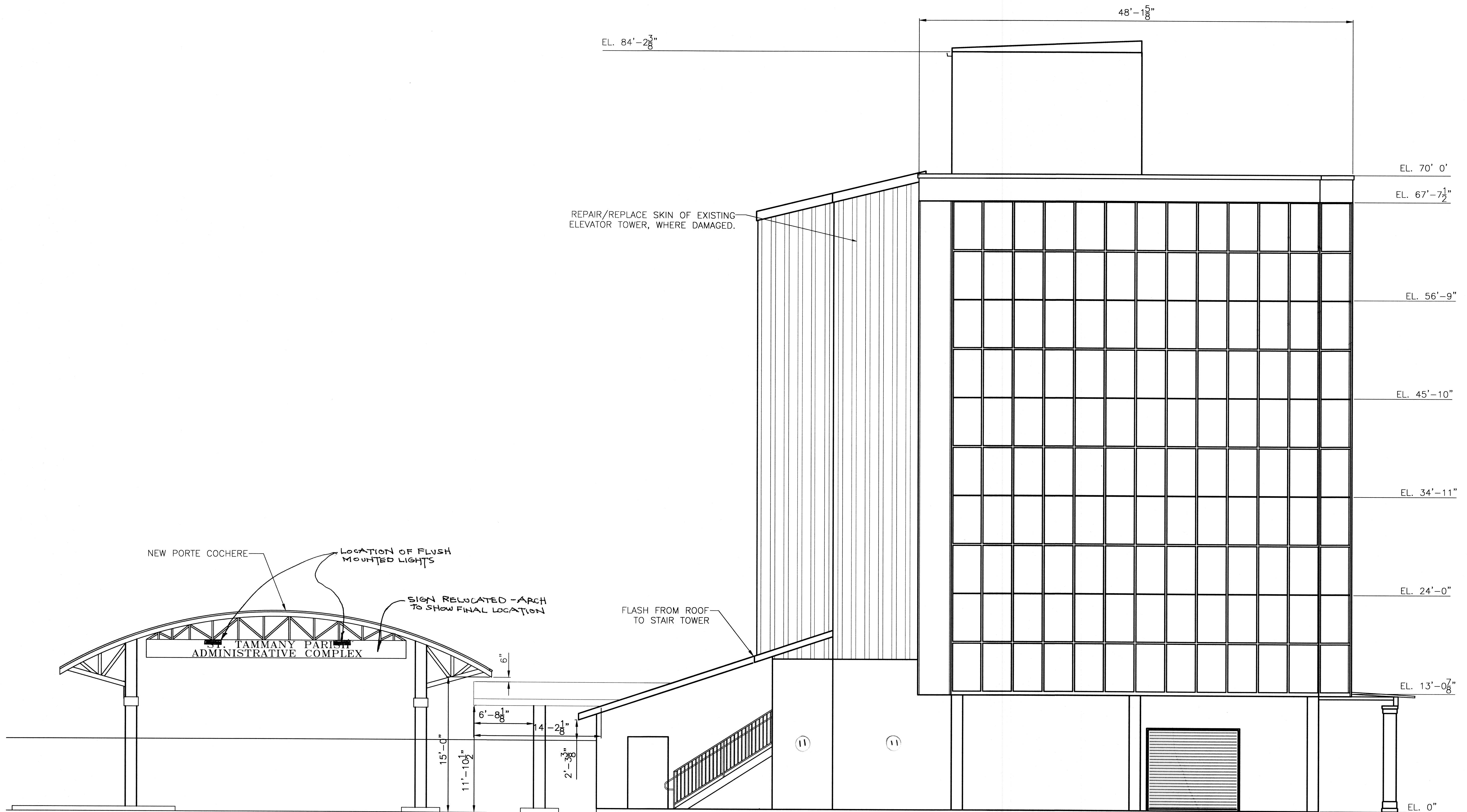
WEST ELEVATION SCALE: 3/16" = 1'-0"
