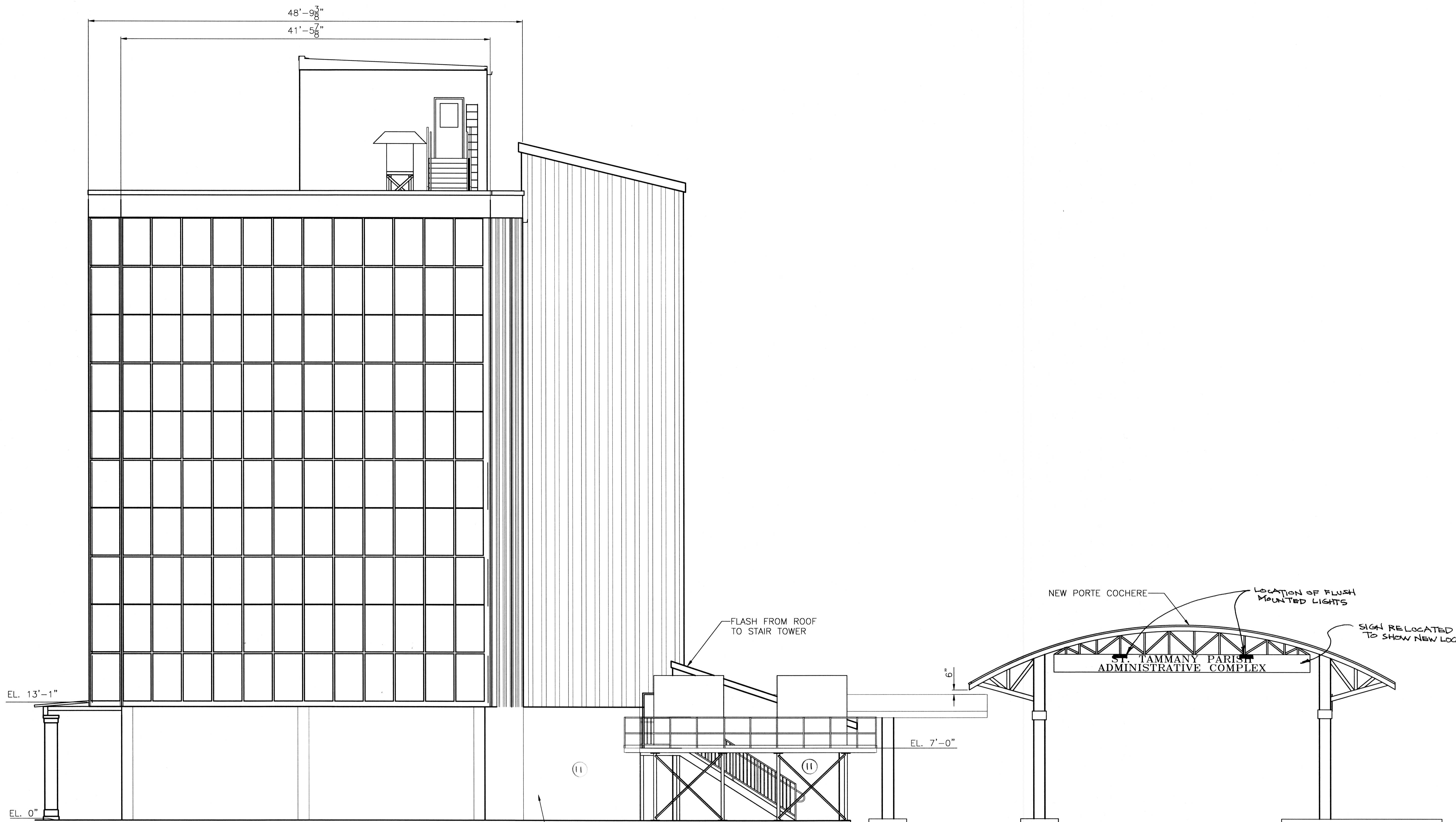
EAST ELEVATION SCALE: 3/16" = 1'-0"
